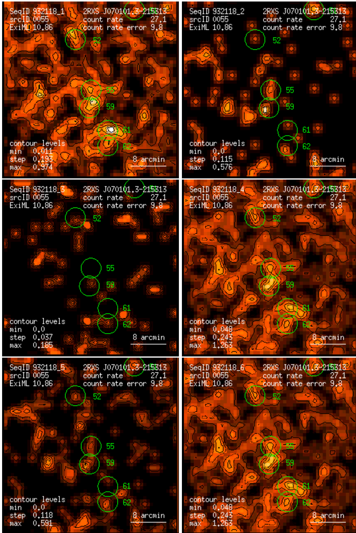
Figure 55: RASS 932118: detection 0055: band rate images, Gaussian filter: (1) PSPC channels 11 – 41, (2) 52 – 90, (3) 91 – 201, (4) 11 – 235, (5) 52 – 201, (6) 11 – 201. Broad band rates in counts/ks. Band rate contour levels in counts/ks/arcmin 2 .
