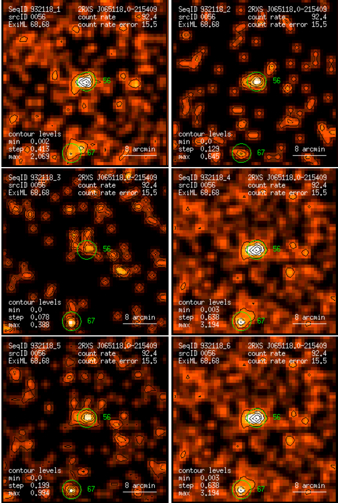
Figure 56: RASS 932118: detection 0056: band rate images, Gaussian filter: (1) PSPC channels 11 – 41, (2) 52 – 90, (3) 91 – 201, (4) 11 – 235, (5) 52 – 201, (6) 11 – 201. Broad band rates in counts/ks. Band rate contour levels in counts/ks/arcmin 2 .
