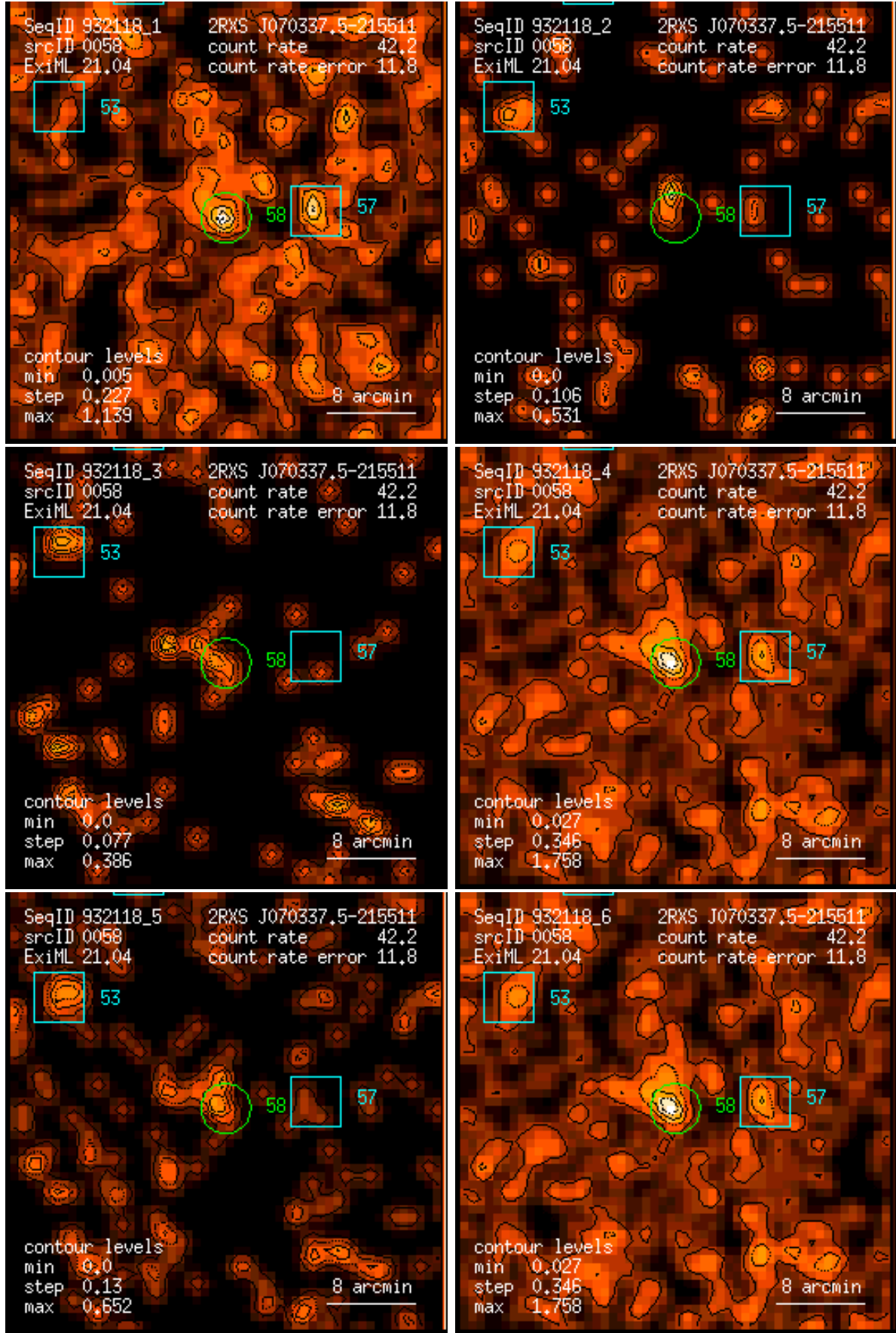
Figure 58: RASS 932118: detection 0058: band rate images, Gaussian filter: (1) PSPC channels 11 – 41, (2) 52 – 90, (3) 91 – 201, (4) 11 – 235, (5) 52 – 201, (6) 11 – 201. Broad band rates in counts/ks. Band rate contour levels in counts/ks/arcmin 2 .
