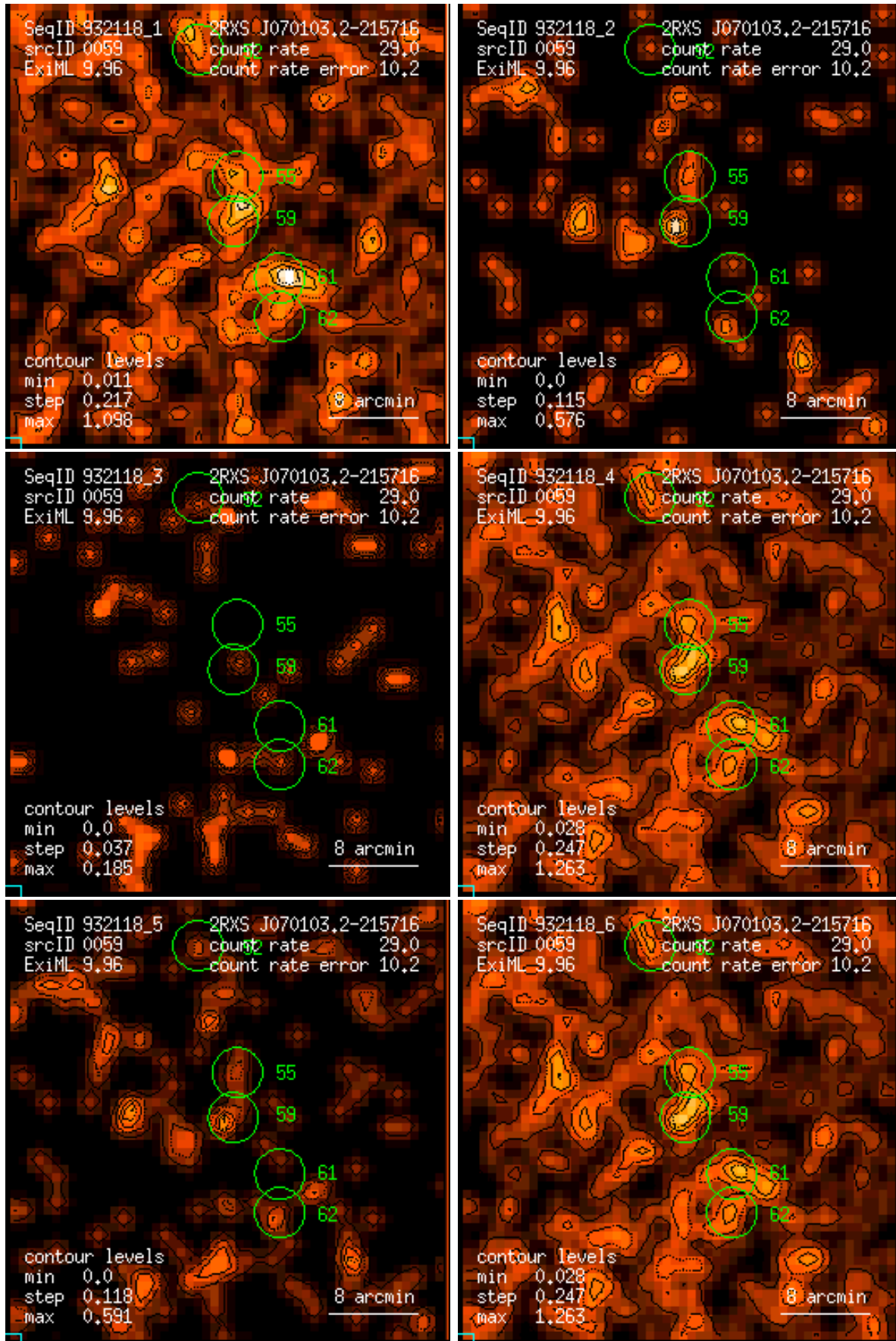
Figure 59: RASS 932118: detection 0059: band rate images, Gaussian filter: (1) PSPC channels 11 – 41, (2) 52 – 90, (3) 91 – 201, (4) 11 – 235, (5) 52 – 201, (6) 11 – 201. Broad band rates in counts/ks. Band rate contour levels in counts/ks/arcmin 2 .
