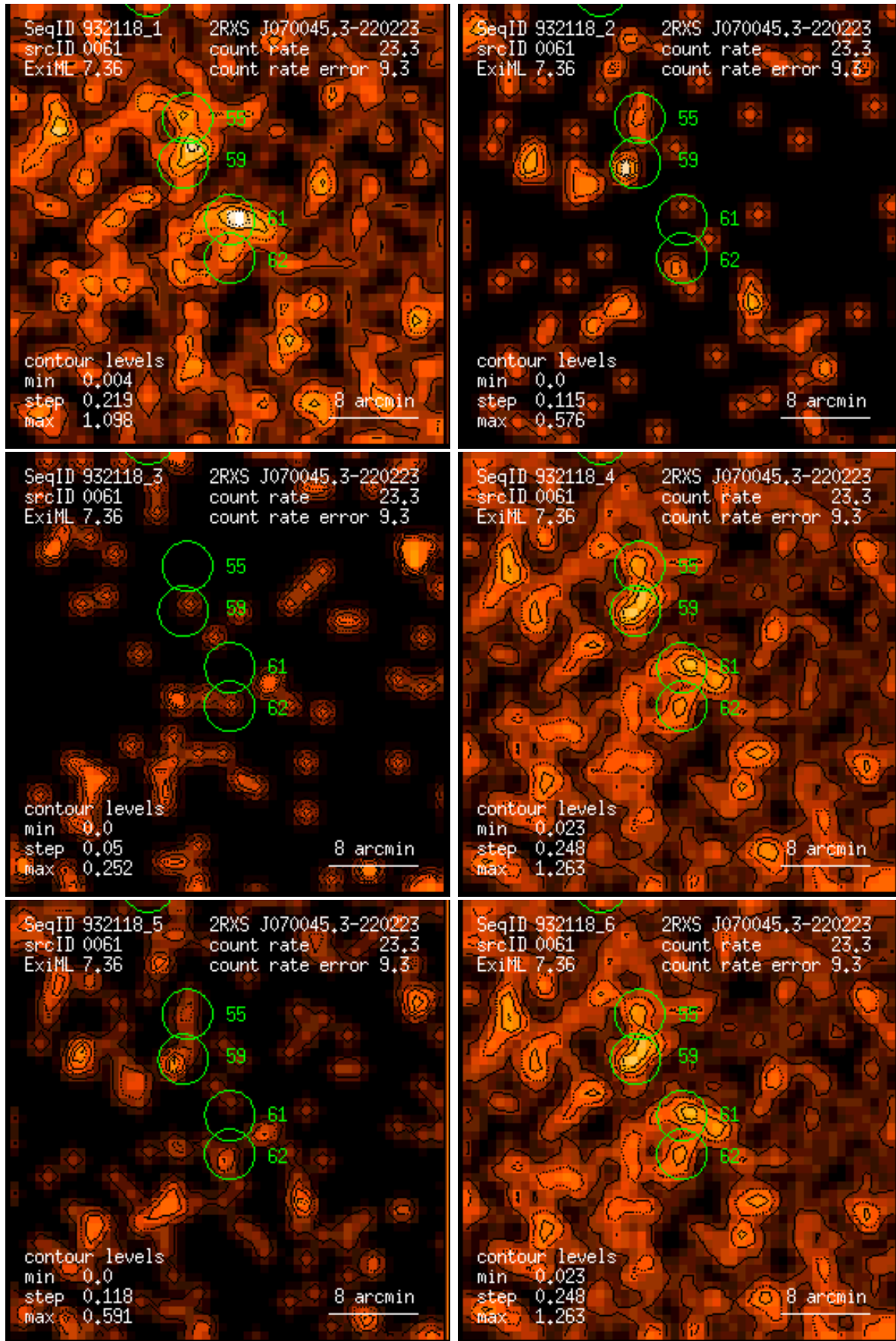
Figure 61: RASS 932118: detection 0061: band rate images, Gaussian filter: (1) PSPC channels 11 – 41, (2) 52 – 90, (3) 91 – 201, (4) 11 – 235, (5) 52 – 201, (6) 11 – 201. Broad band rates in counts/ks. Band rate contour levels in counts/ks/arcmin 2 .
