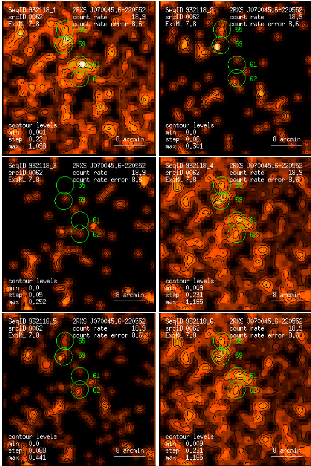
Figure 62: RASS 932118: detection 0062: band rate images, Gaussian filter: (1) PSPC channels 11 – 41, (2) 52 – 90, (3) 91 – 201, (4) 11 – 235, (5) 52 – 201, (6) 11 – 201. Broad band rates in counts/ks. Band rate contour levels in counts/ks/arcmin 2 .
