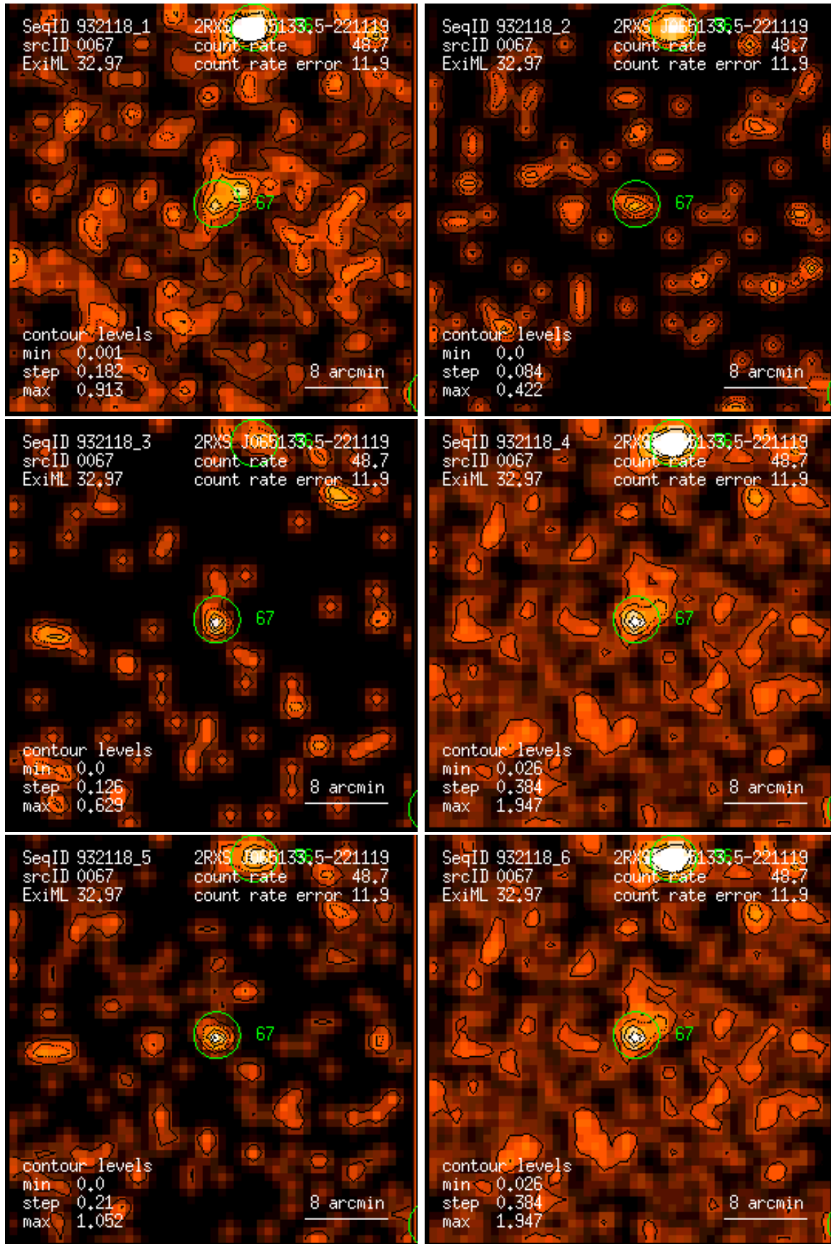
Figure 67: RASS 932118: detection 0067: band rate images, Gaussian filter: (1) PSPC channels 11 – 41, (2) 52 – 90, (3) 91 – 201, (4) 11 – 235, (5) 52 – 201, (6) 11 – 201. Broad band rates in counts/ks. Band rate contour levels in counts/ks/arcmin 2 .
