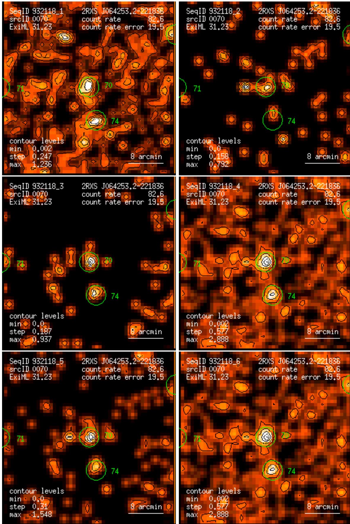
Figure 70: RASS 932118: detection 0070: band rate images, Gaussian filter: (1) PSPC channels 11 – 41, (2) 52 – 90, (3) 91 – 201, (4) 11 – 235, (5) 52 – 201, (6) 11 – 201. Broad band rates in counts/ks. Band rate contour levels in counts/ks/arcmin 2 .
