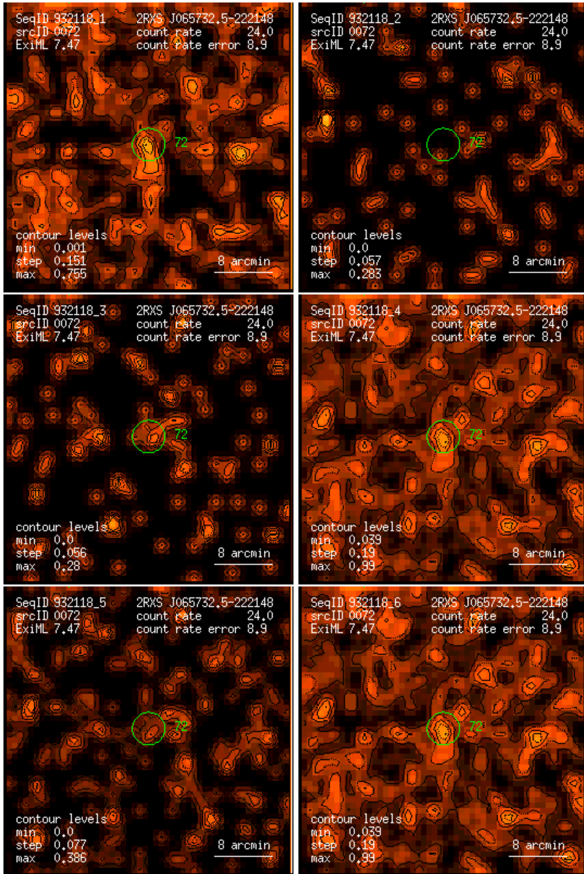
Figure 72: RASS 932118: detection 0072: band rate images, Gaussian filter: (1) PSPC channels 11 – 41, (2) 52 – 90, (3) 91 – 201, (4) 11 – 235, (5) 52 – 201, (6) 11 – 201. Broad band rates in counts/ks. Band rate contour levels in counts/ks/arcmin 2 .
