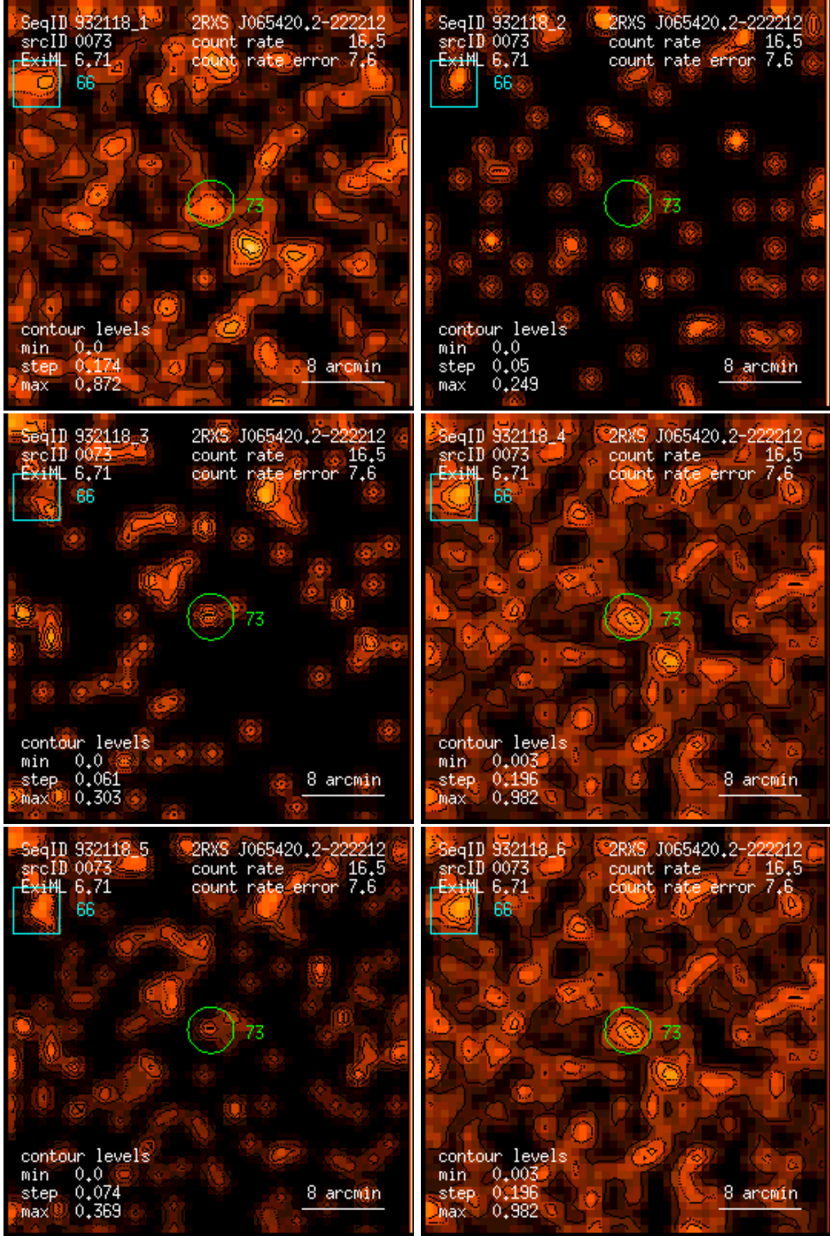
Figure 73: RASS 932118: detection 0073: band rate images, Gaussian filter: (1) PSPC channels 11 – 41, (2) 52 – 90, (3) 91 – 201, (4) 11 – 235, (5) 52 – 201, (6) 11 – 201. Broad band rates in counts/ks. Band rate contour levels in counts/ks/arcmin 2 .
