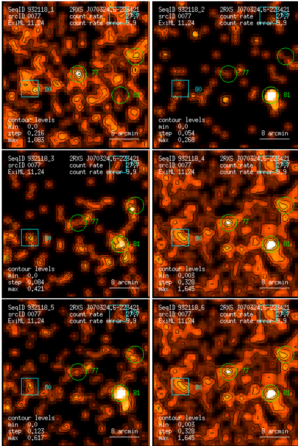
Figure 77: RASS 932118: detection 0077: band rate images, Gaussian filter: (1) PSPC channels 11 – 41, (2) 52 – 90, (3) 91 – 201, (4) 11 – 235, (5) 52 – 201, (6) 11 – 201. Broad band rates in counts/ks. Band rate contour levels in counts/ks/arcmin 2 .
