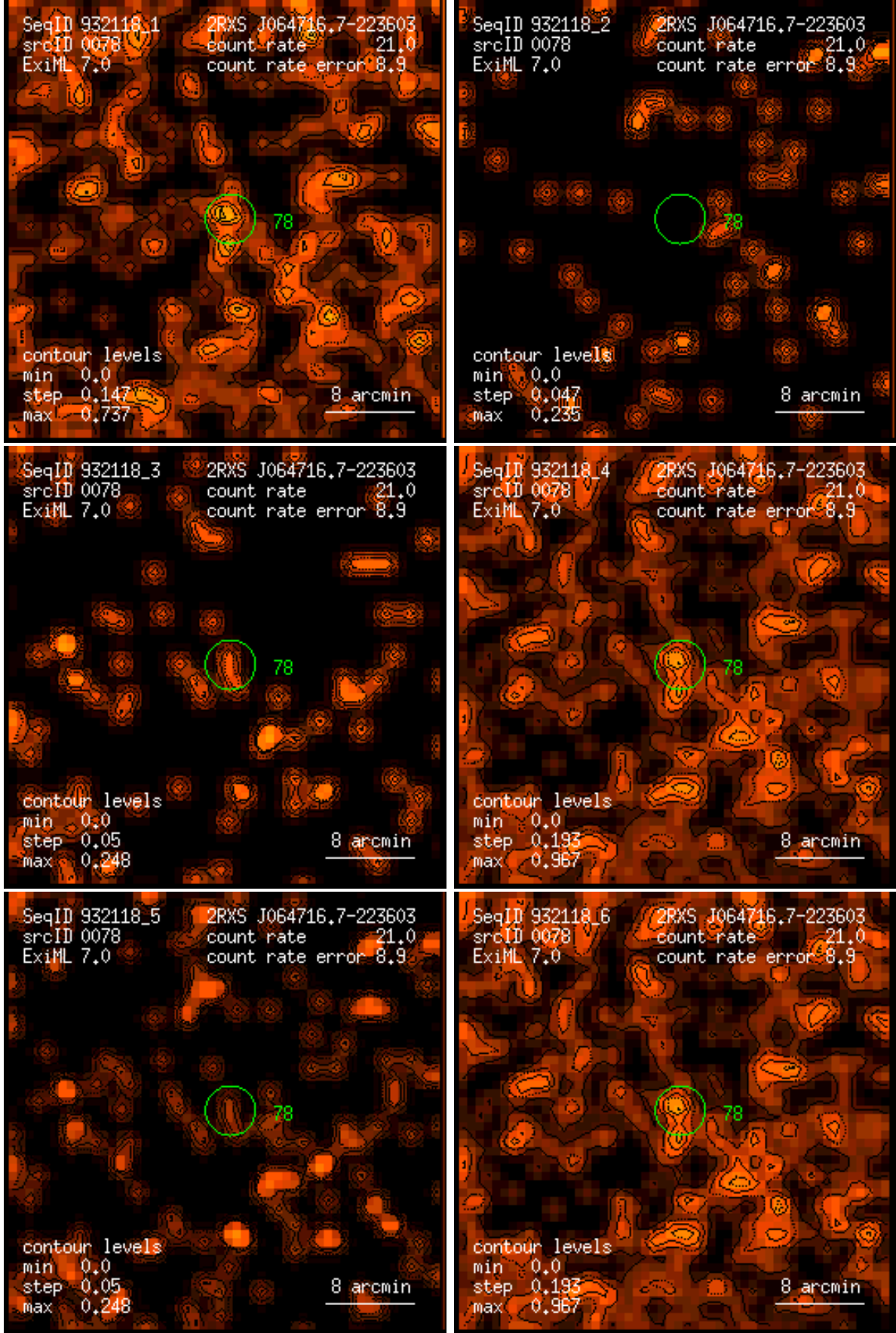
Figure 78: RASS 932118: detection 0078: band rate images, Gaussian filter: (1) PSPC channels 11 – 41, (2) 52 – 90, (3) 91 – 201, (4) 11 – 235, (5) 52 – 201, (6) 11 – 201. Broad band rates in counts/ks. Band rate contour levels in counts/ks/arcmin 2 .
