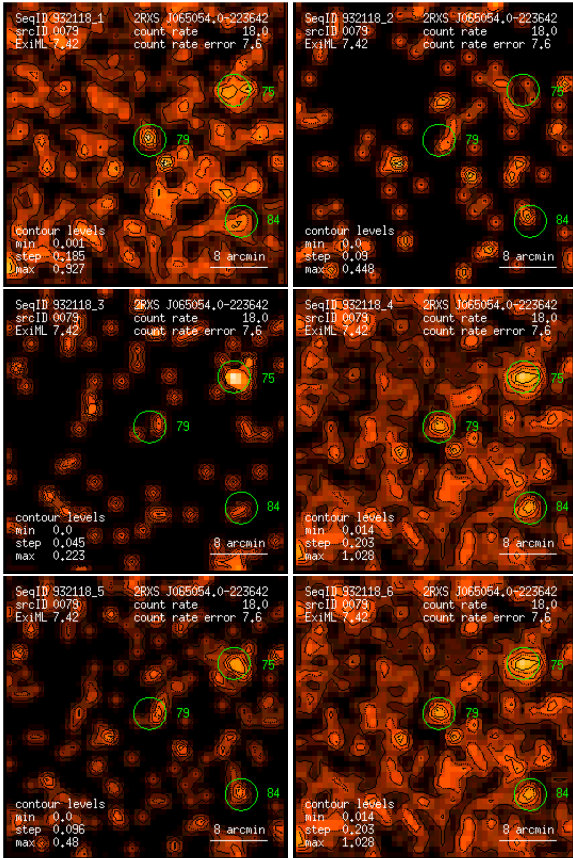
Figure 79: RASS 932118: detection 0079: band rate images, Gaussian filter: (1) PSPC channels 11 – 41, (2) 52 – 90, (3) 91 – 201, (4) 11 – 235, (5) 52 – 201, (6) 11 – 201. Broad band rates in counts/ks. Band rate contour levels in counts/ks/arcmin 2 .
