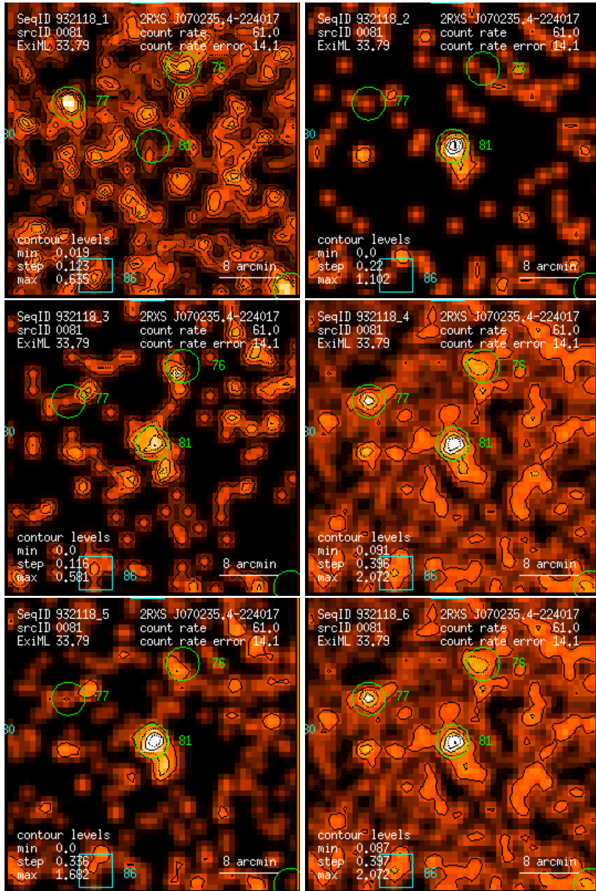
Figure 81: RASS 932118: detection 0081: band rate images, Gaussian filter: (1) PSPC channels 11 – 41, (2) 52 – 90, (3) 91 – 201, (4) 11 – 235, (5) 52 – 201, (6) 11 – 201. Broad band rates in counts/ks. Band rate contour levels in counts/ks/arcmin 2 .
