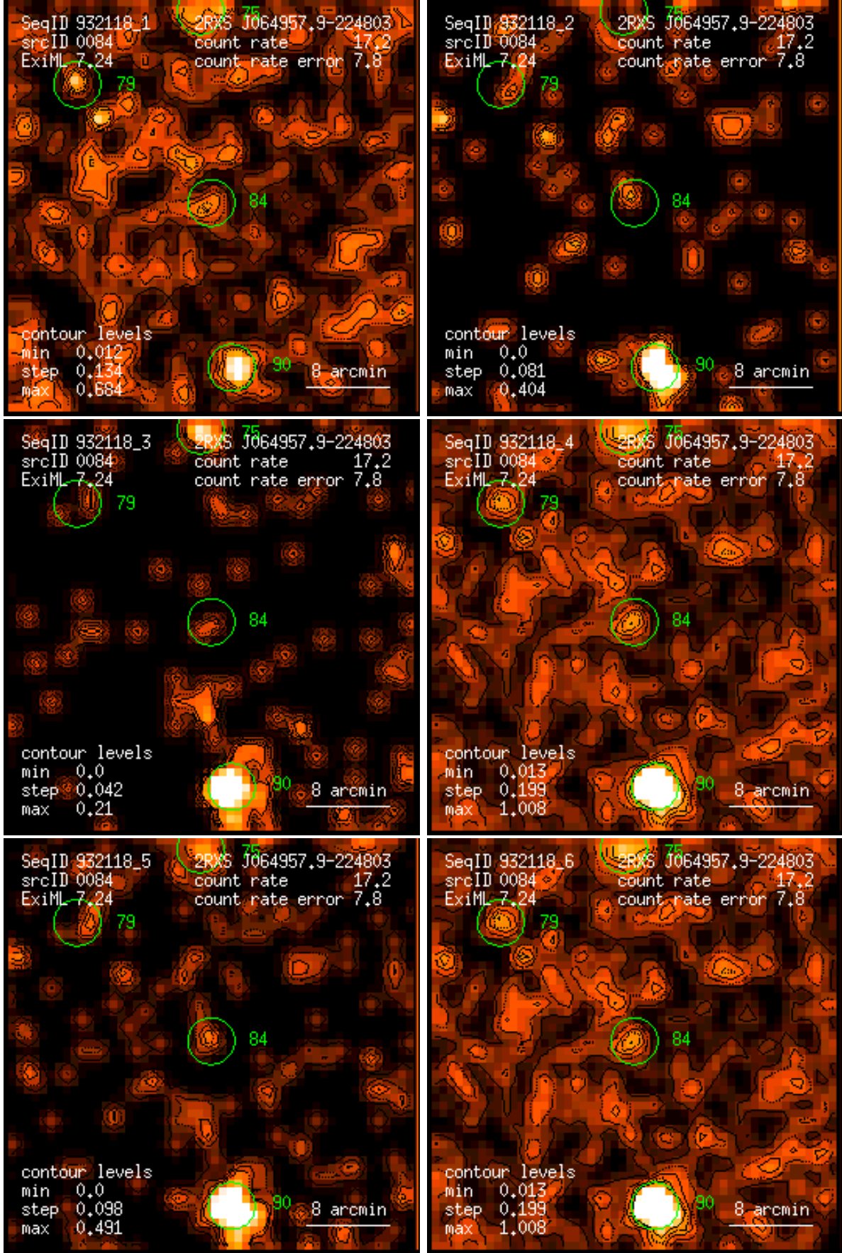
Figure 84: RASS 932118: detection 0084: band rate images, Gaussian filter: (1) PSPC channels 11 – 41, (2) 52 – 90, (3) 91 – 201, (4) 11 – 235, (5) 52 – 201, (6) 11 – 201. Broad band rates in counts/ks. Band rate contour levels in counts/ks/arcmin 2 .
