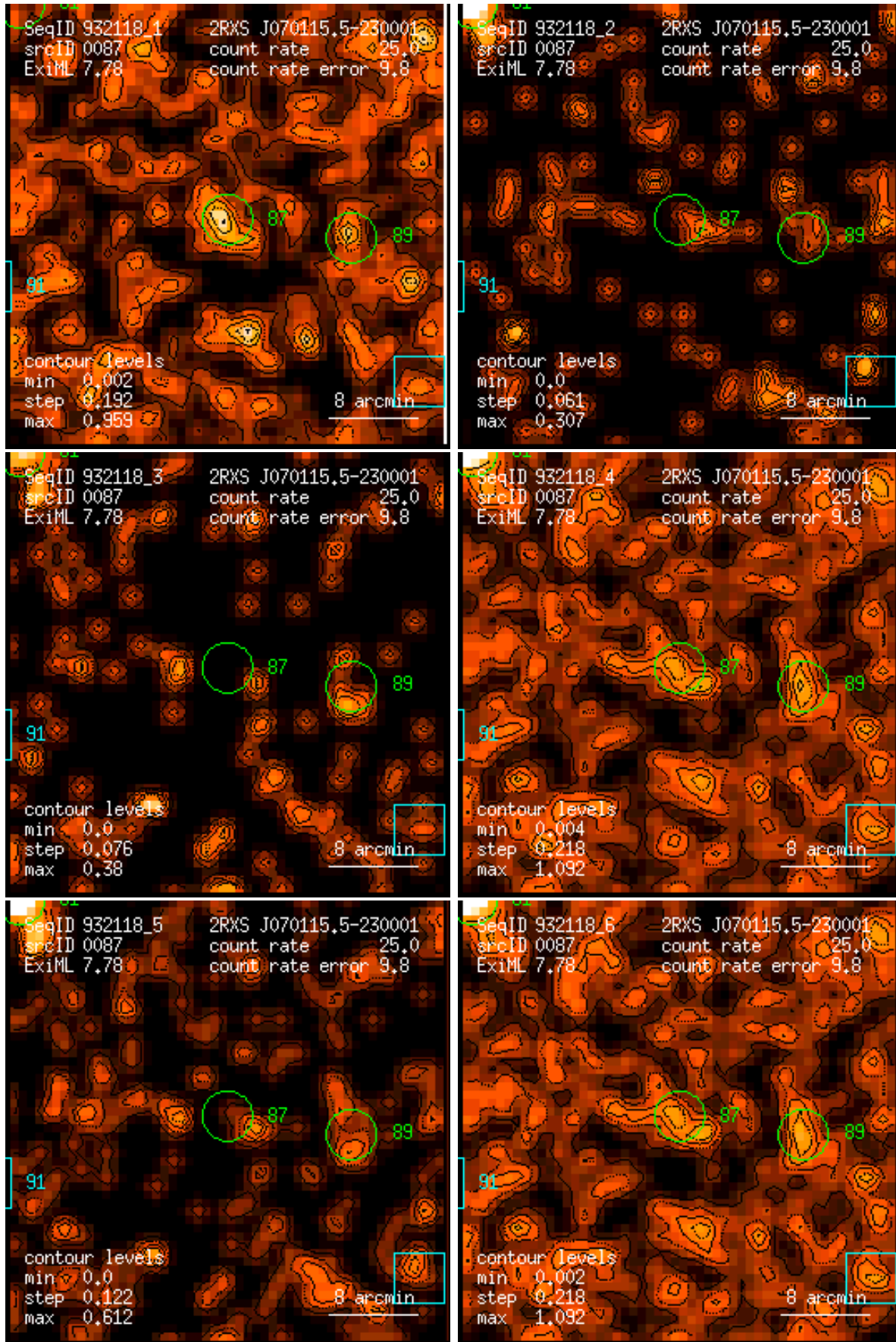
Figure 87: RASS 932118: detection 0087: band rate images, Gaussian filter: (1) PSPC channels 11 – 41, (2) 52 – 90, (3) 91 – 201, (4) 11 – 235, (5) 52 – 201, (6) 11 – 201. Broad band rates in counts/ks. Band rate contour levels in counts/ks/arcmin 2 .
