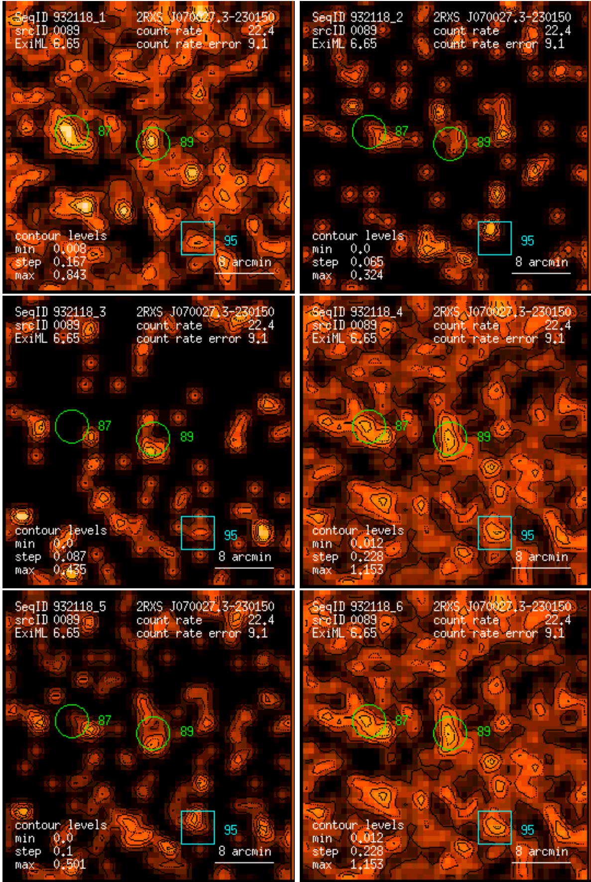
Figure 89: RASS 932118: detection 0089: band rate images, Gaussian filter: (1) PSPC channels 11 – 41, (2) 52 – 90, (3) 91 – 201, (4) 11 – 235, (5) 52 – 201, (6) 11 – 201. Broad band rates in counts/ks. Band rate contour levels in counts/ks/arcmin 2 .
