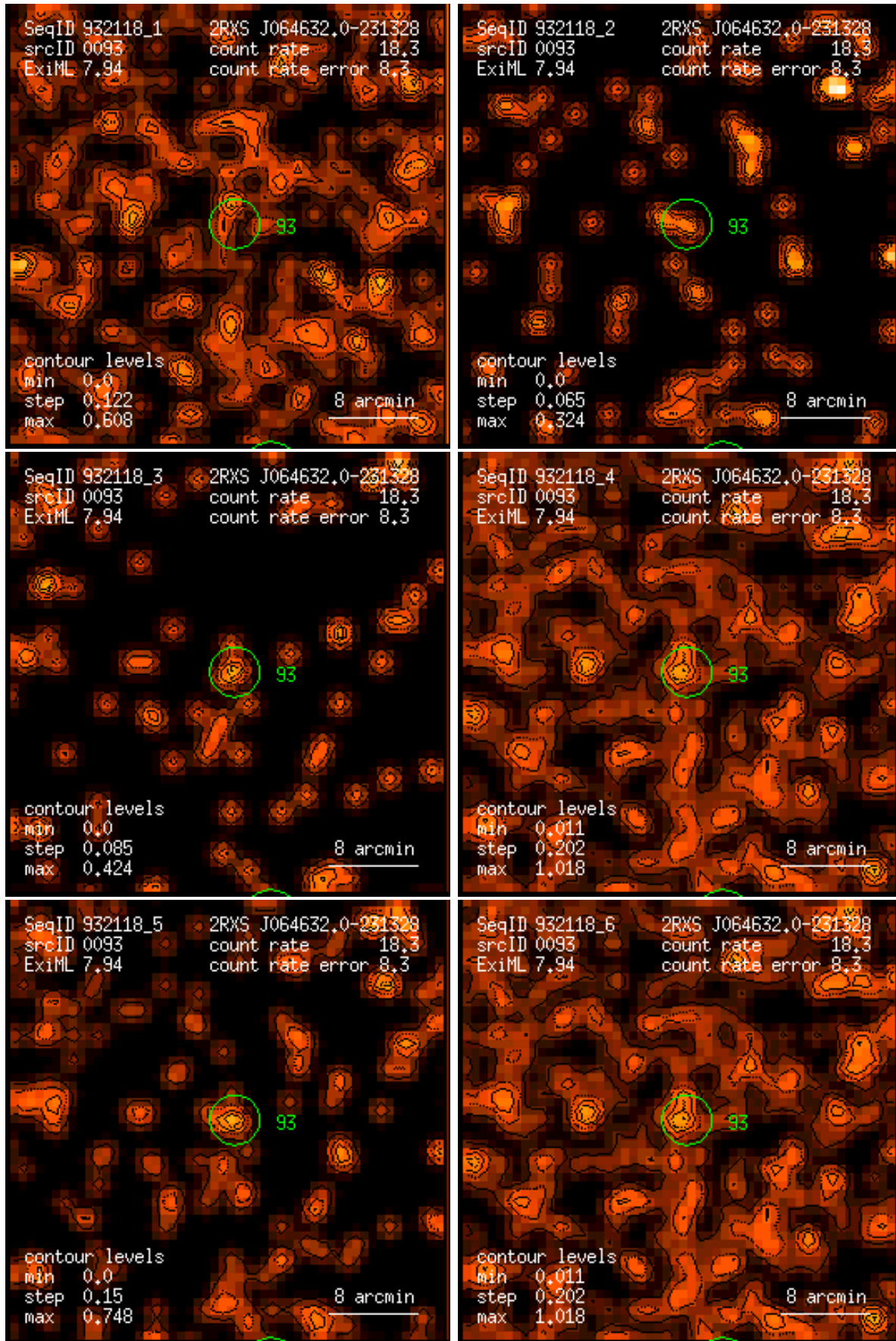
Figure 93: RASS 932118: detection 0093: band rate images, Gaussian filter: (1) PSPC channels 11 – 41, (2) 52 – 90, (3) 91 – 201, (4) 11 – 235, (5) 52 – 201, (6) 11 – 201. Broad band rates in counts/ks. Band rate contour levels in counts/ks/arcmin 2 .
