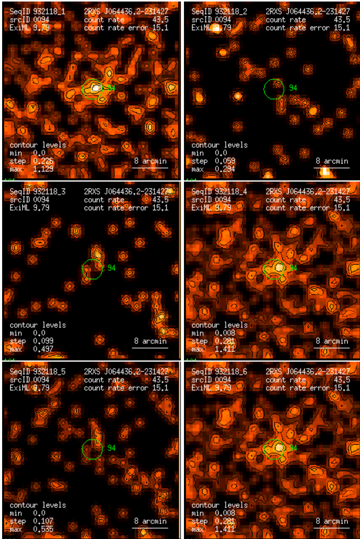
Figure 94: RASS 932118: detection 0094: band rate images, Gaussian filter: (1) PSPC channels 11 – 41, (2) 52 – 90, (3) 91 – 201, (4) 11 – 235, (5) 52 – 201, (6) 11 – 201. Broad band rates in counts/ks. Band rate contour levels in counts/ks/arcmin 2 .
