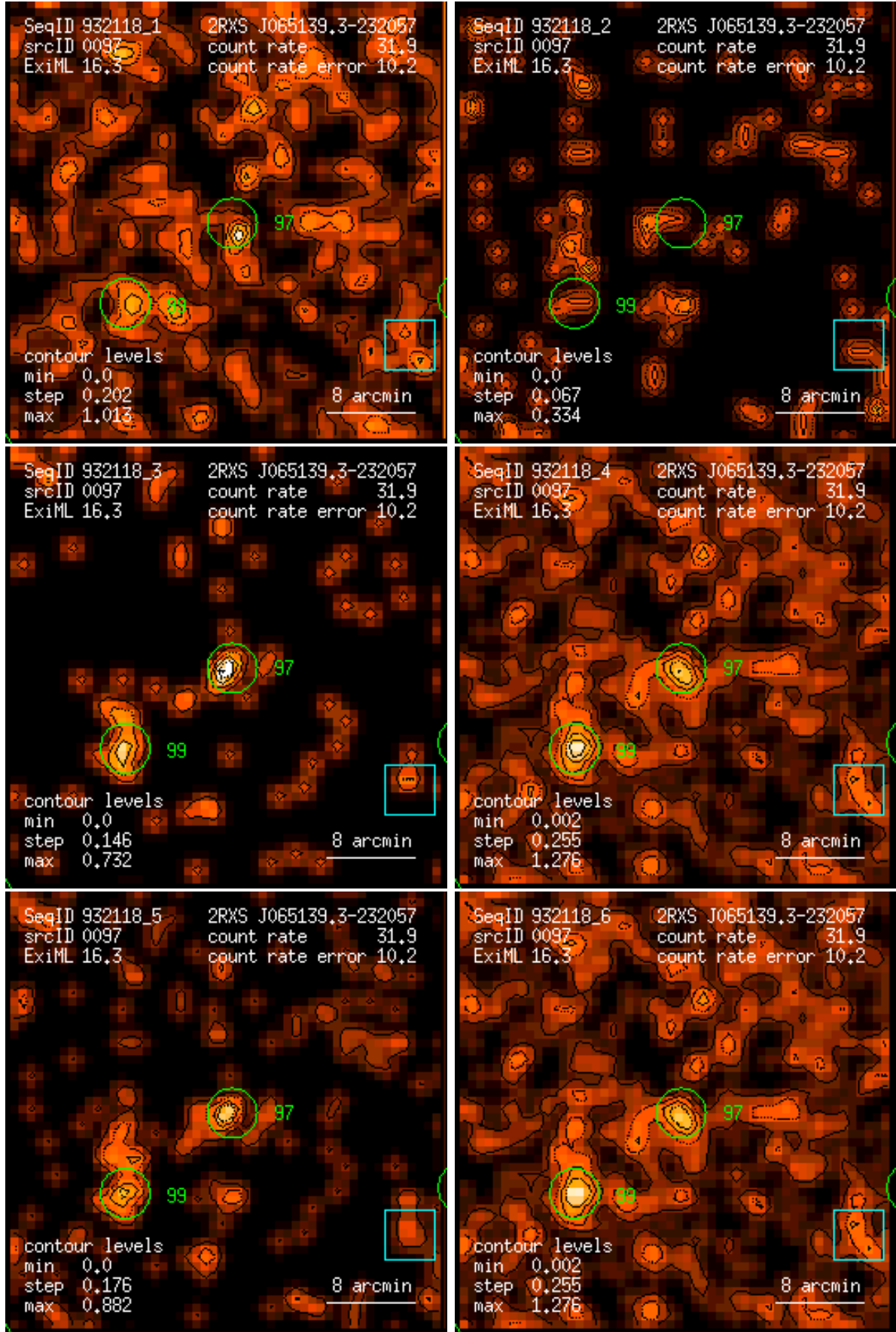
Figure 97: RASS 932118: detection 0097: band rate images, Gaussian filter: (1) PSPC channels 11 – 41, (2) 52 – 90, (3) 91 – 201, (4) 11 – 235, (5) 52 – 201, (6) 11 – 201. Broad band rates in counts/ks. Band rate contour levels in counts/ks/arcmin 2 .
