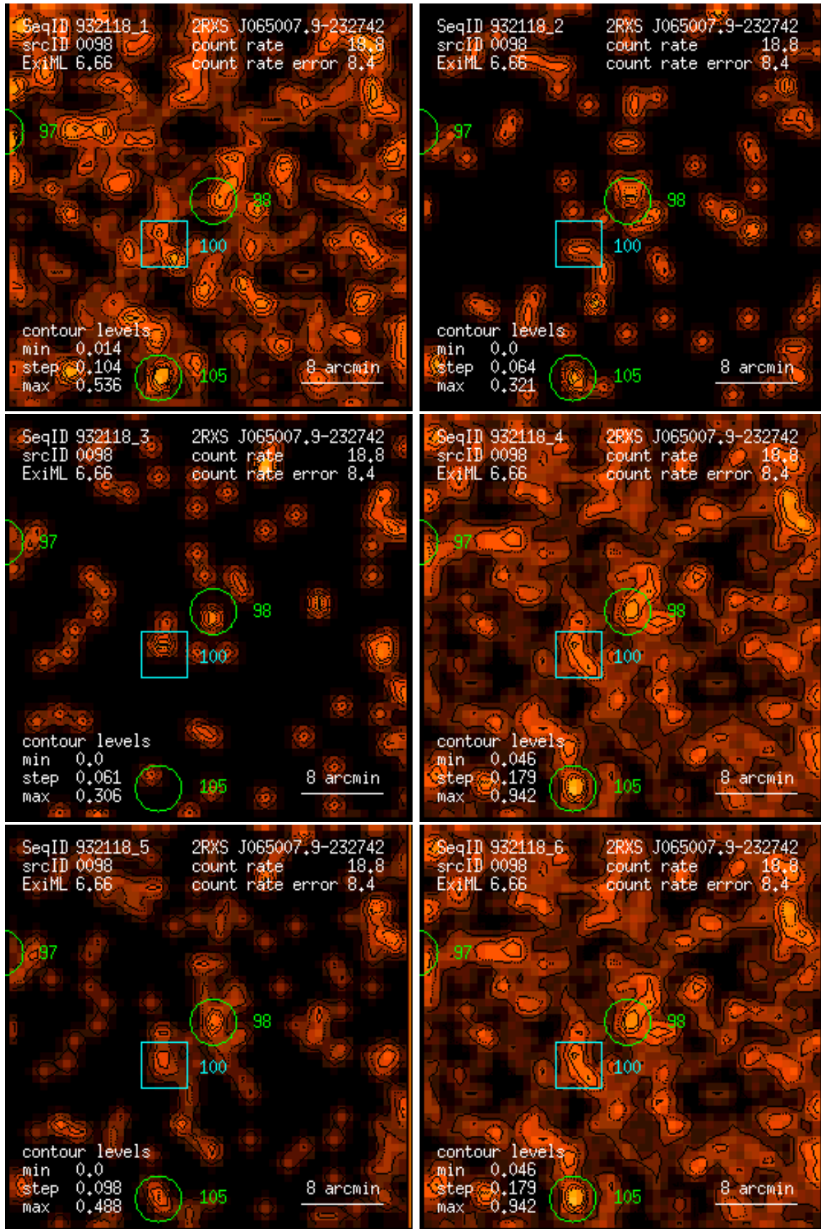
Figure 98: RASS 932118: detection 0098: band rate images, Gaussian filter: (1) PSPC channels 11 – 41, (2) 52 – 90, (3) 91 – 201, (4) 11 – 235, (5) 52 – 201, (6) 11 – 201. Broad band rates in counts/ks. Band rate contour levels in counts/ks/arcmin 2 .
