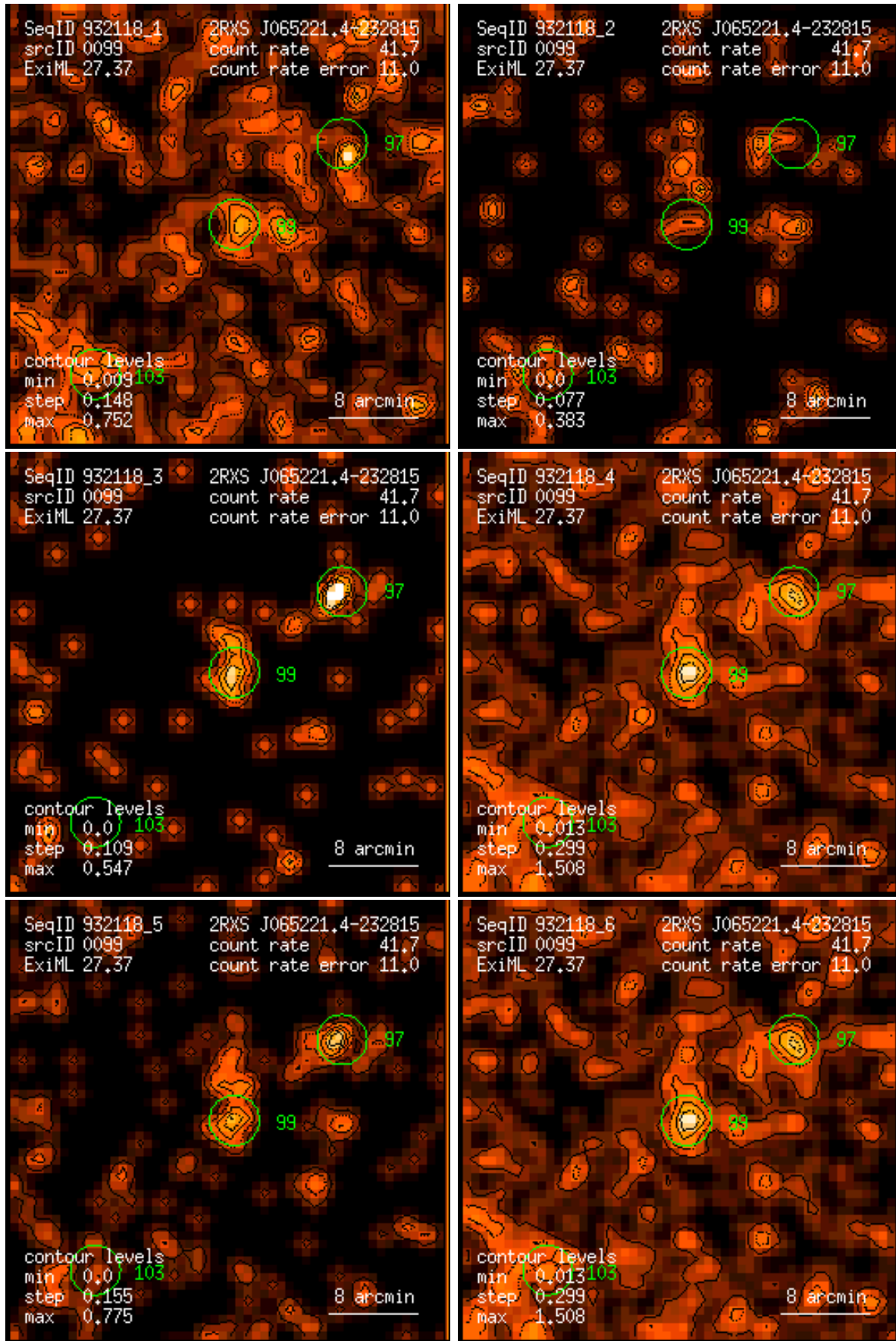
Figure 99: RASS 932118: detection 0099: band rate images, Gaussian filter: (1) PSPC channels 11 – 41, (2) 52 – 90, (3) 91 – 201, (4) 11 – 235, (5) 52 – 201, (6) 11 – 201. Broad band rates in counts/ks. Band rate contour levels in counts/ks/arcmin 2 .
