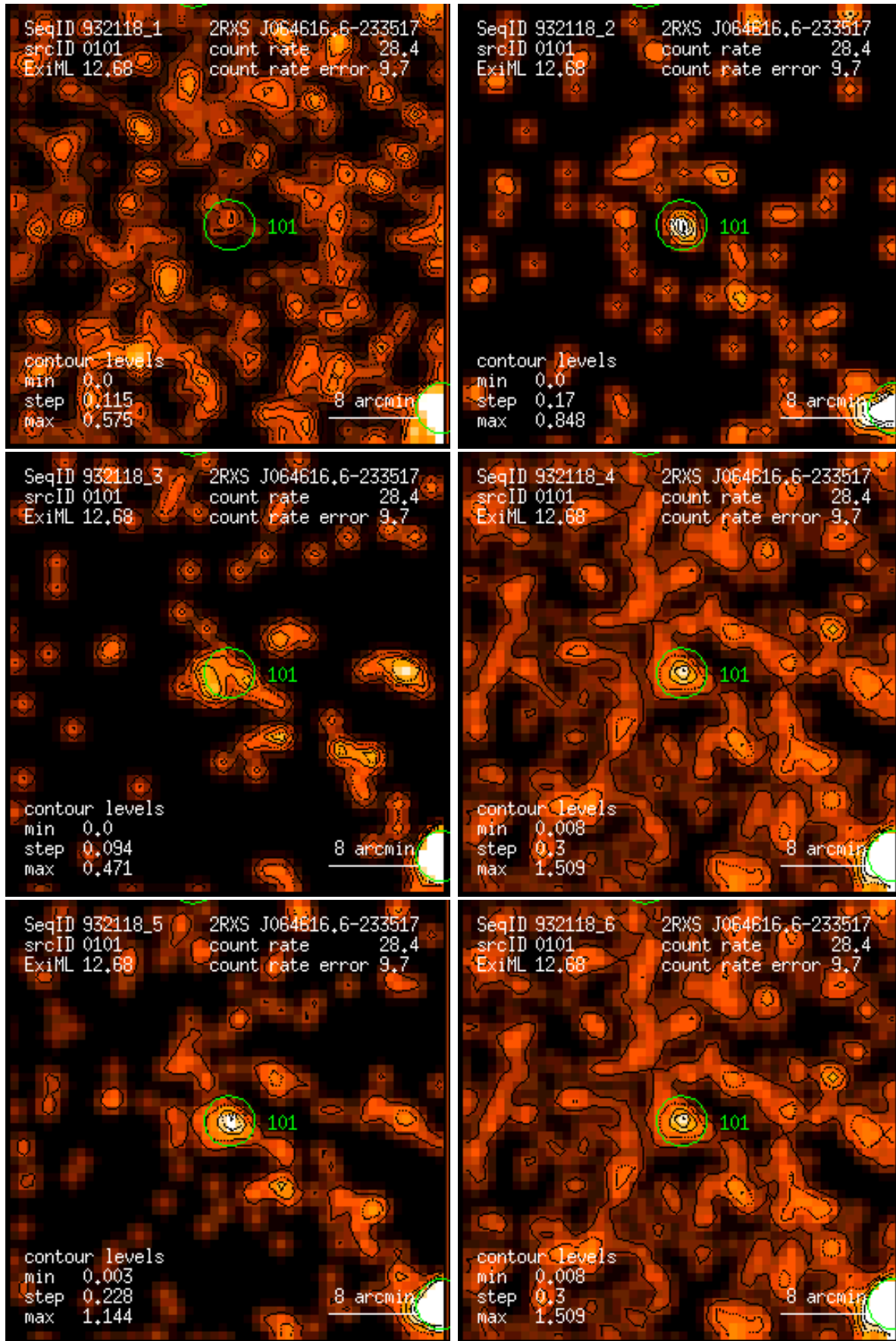
Figure 101: RASS 932118: detection 0101: band rate images, Gaussian filter: (1) PSPC channels 11 – 41, (2) 52 – 90, (3) 91 – 201, (4) 11 – 235, (5) 52 – 201, (6) 11 – 201. Broad band rates in counts/ks. Band rate contour levels in counts/ks/arcmin 2 .
