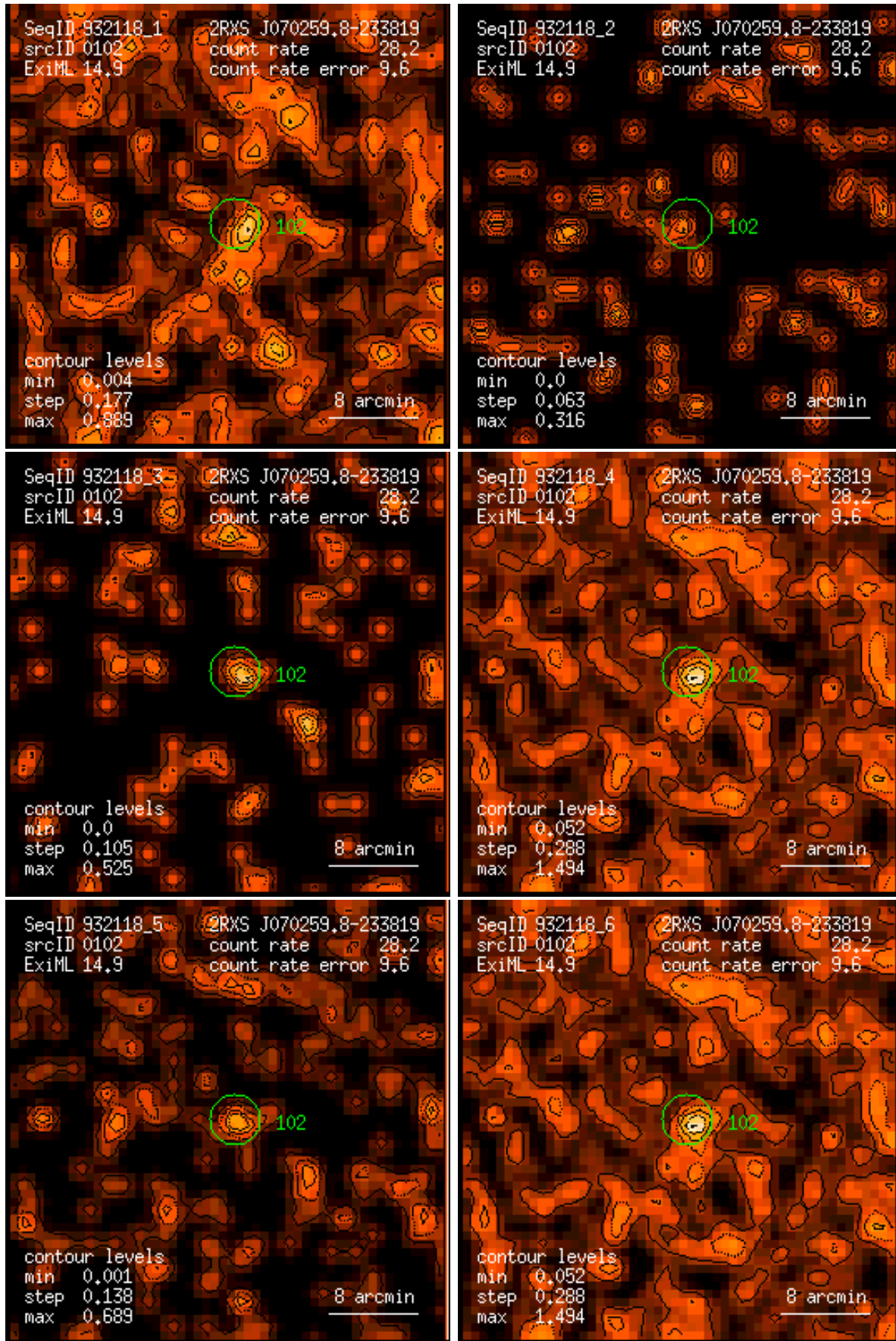
Figure 102: RASS 932118: detection 0102: band rate images, Gaussian filter: (1) PSPC channels 11 – 41, (2) 52 – 90, (3) 91 – 201, (4) 11 – 235, (5) 52 – 201, (6) 11 – 201. Broad band rates in counts/ks. Band rate contour levels in counts/ks/arcmin 2 .
