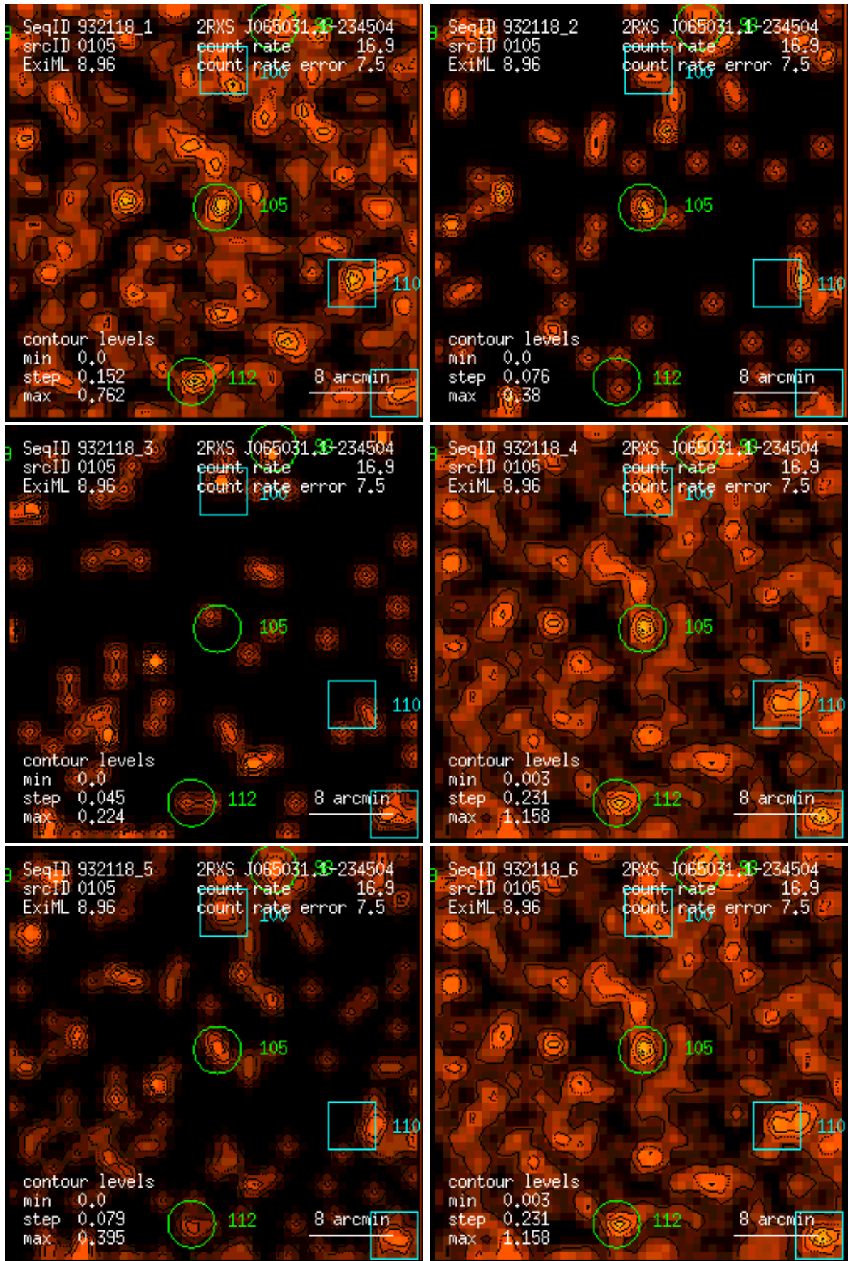
Figure 105: RASS 932118: detection 0105: band rate images, Gaussian filter: (1) PSPC channels 11 – 41, (2) 52 – 90, (3) 91 – 201, (4) 11 – 235, (5) 52 – 201, (6) 11 – 201. Broad band rates in counts/ks. Band rate contour levels in counts/ks/arcmin 2 .
