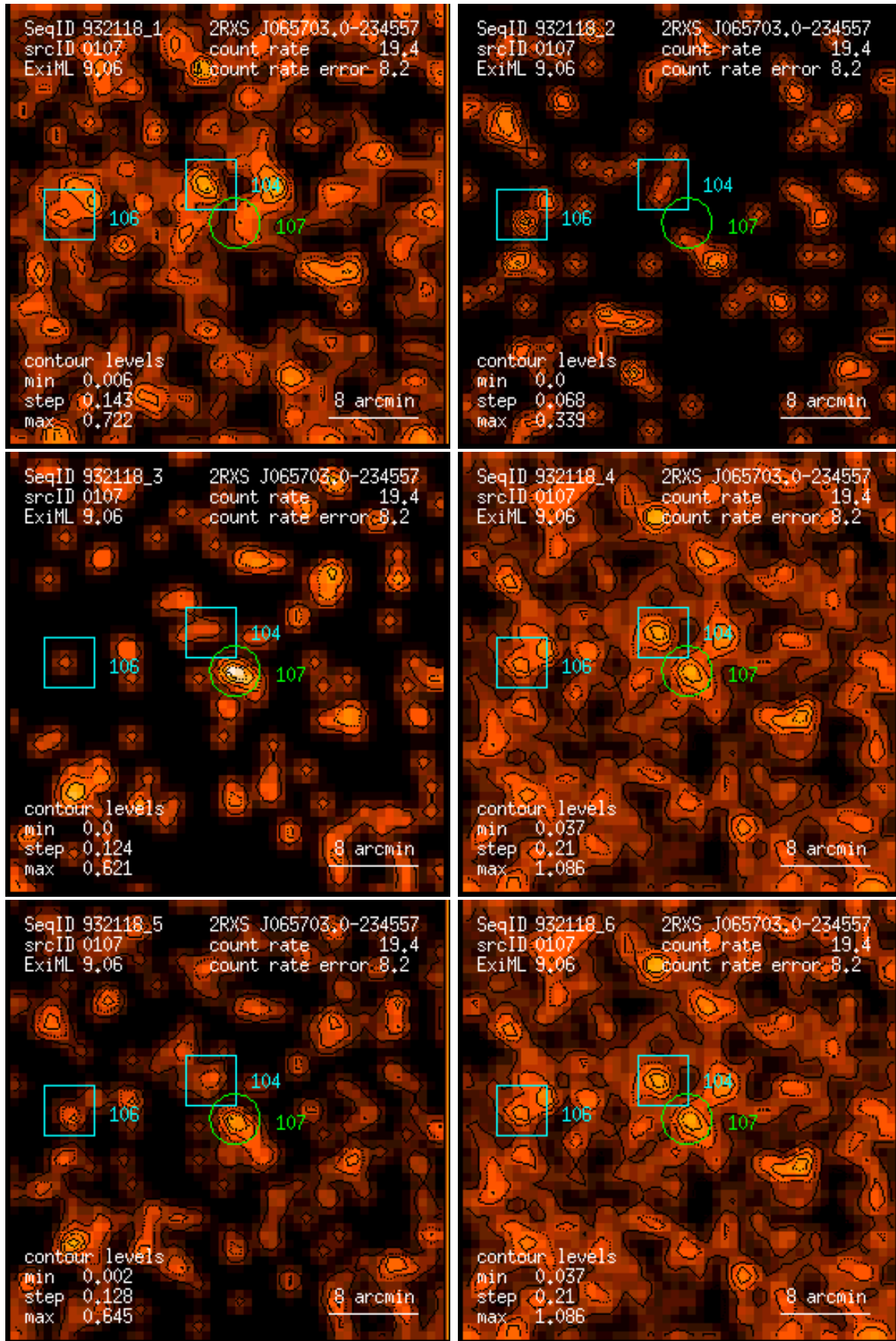
Figure 107: RASS 932118: detection 0107: band rate images, Gaussian filter: (1) PSPC channels 11 – 41, (2) 52 – 90, (3) 91 – 201, (4) 11 – 235, (5) 52 – 201, (6) 11 – 201. Broad band rates in counts/ks. Band rate contour levels in counts/ks/arcmin 2 .
