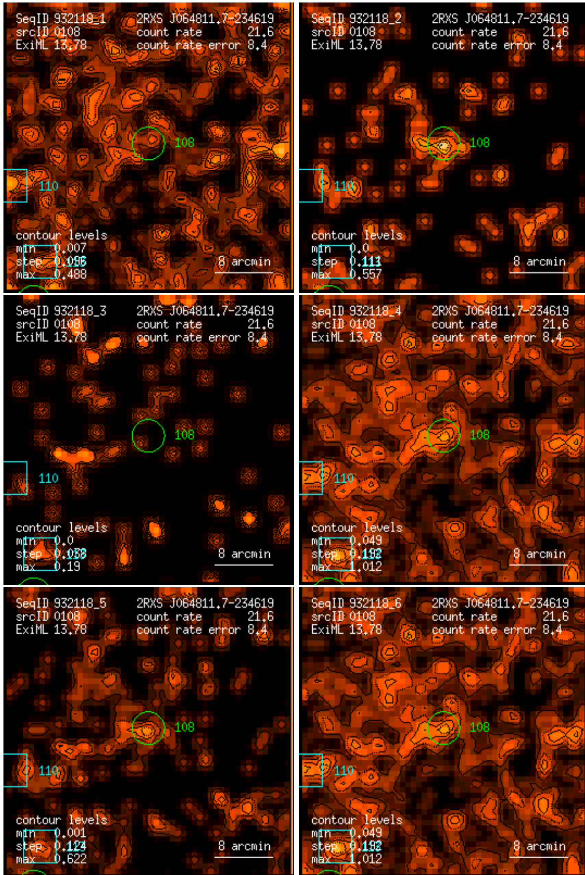
Figure 108: RASS 932118: detection 0108: band rate images, Gaussian filter: (1) PSPC channels 11 – 41, (2) 52 – 90, (3) 91 – 201, (4) 11 – 235, (5) 52 – 201, (6) 11 – 201. Broad band rates in counts/ks. Band rate contour levels in counts/ks/arcmin 2 .
