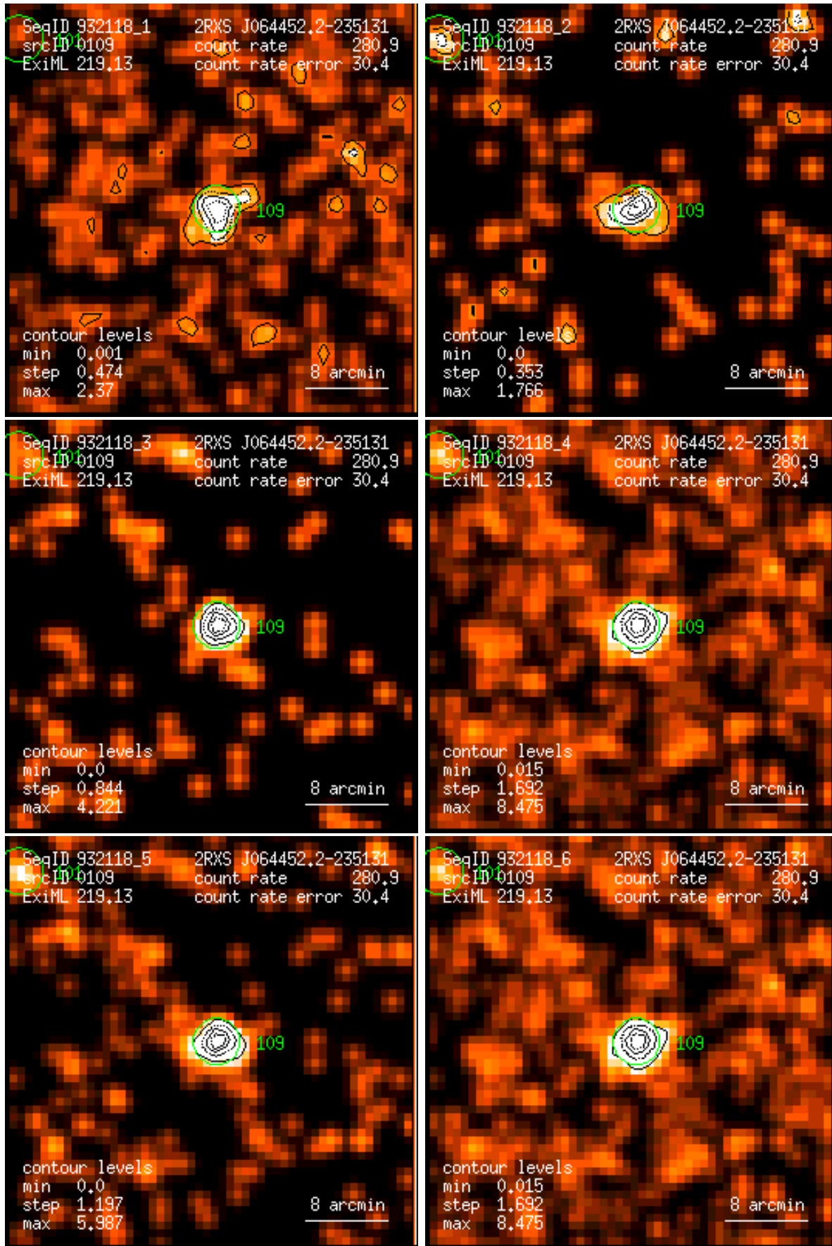
Figure 109: RASS 932118: detection 0109: band rate images, Gaussian filter: (1) PSPC channels 11 – 41, (2) 52 – 90, (3) 91 – 201, (4) 11 – 235, (5) 52 – 201, (6) 11 – 201. Broad band rates in counts/ks. Band rate contour levels in counts/ks/arcmin 2 .
