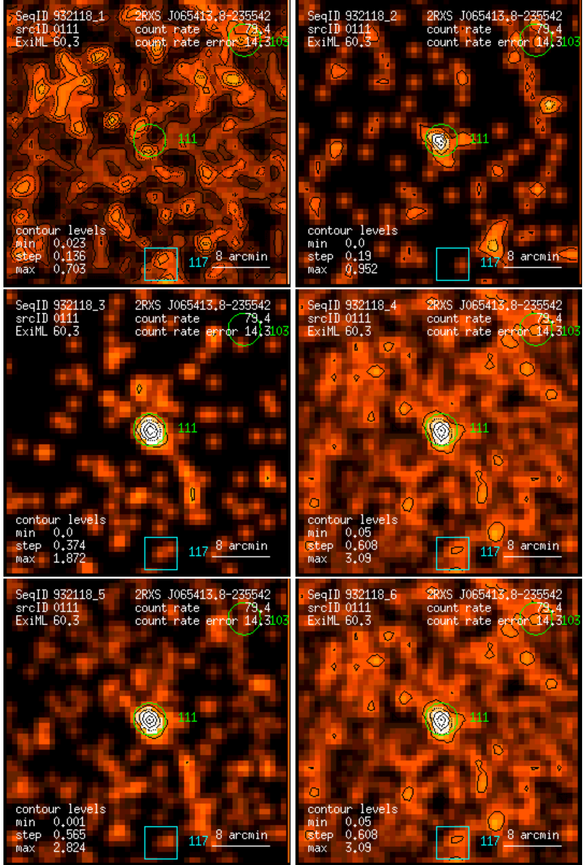
Figure 111: RASS 932118: detection 0111: band rate images, Gaussian filter: (1) PSPC channels 11 – 41, (2) 52 – 90, (3) 91 – 201, (4) 11 – 235, (5) 52 – 201, (6) 11 – 201. Broad band rates in counts/ks. Band rate contour levels in counts/ks/arcmin 2 .
