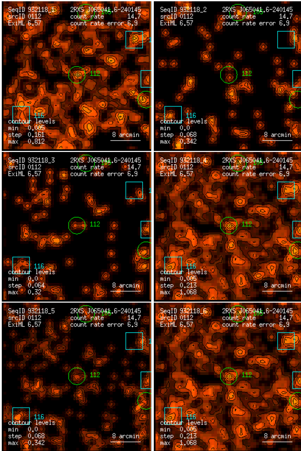
Figure 112: RASS 932118: detection 0112: band rate images, Gaussian filter: (1) PSPC channels 11 – 41, (2) 52 – 90, (3) 91 – 201, (4) 11 – 235, (5) 52 – 201, (6) 11 – 201. Broad band rates in counts/ks. Band rate contour levels in counts/ks/arcmin 2 .
