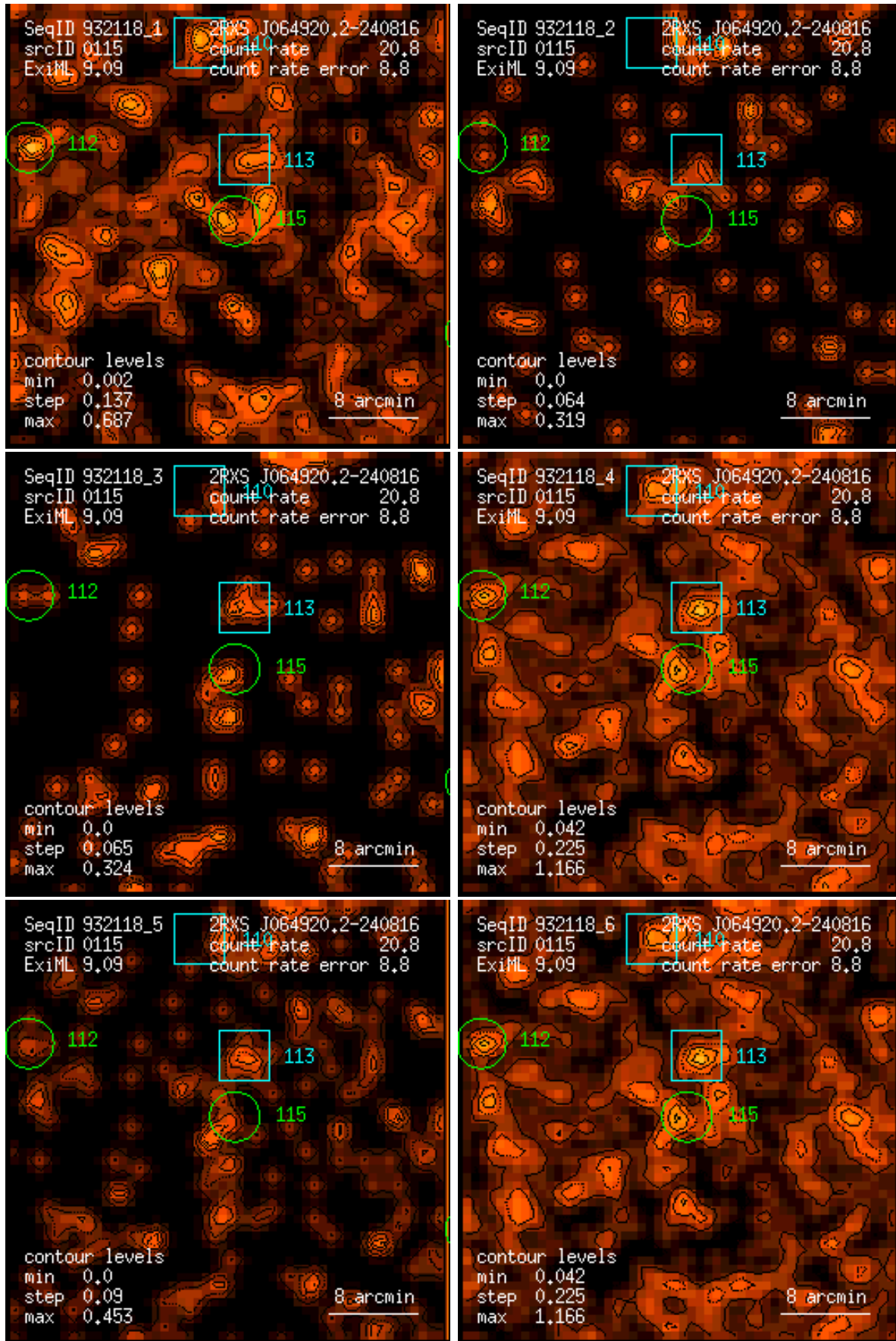
Figure 115: RASS 932118: detection 0115: band rate images, Gaussian filter: (1) PSPC channels 11 – 41, (2) 52 – 90, (3) 91 – 201, (4) 11 – 235, (5) 52 – 201, (6) 11 – 201. Broad band rates in counts/ks. Band rate contour levels in counts/ks/arcmin 2 .
