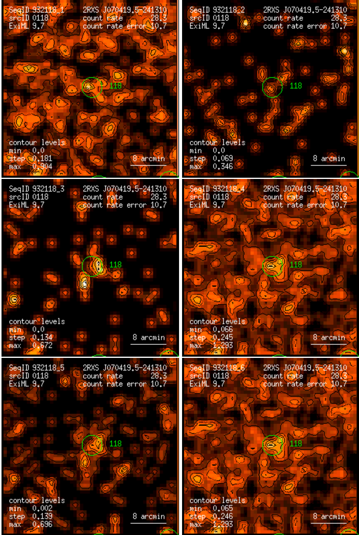
Figure 118: RASS 932118: detection 0118: band rate images, Gaussian filter: (1) PSPC channels 11 – 41, (2) 52 – 90, (3) 91 – 201, (4) 11 – 235, (5) 52 – 201, (6) 11 – 201. Broad band rates in counts/ks. Band rate contour levels in counts/ks/arcmin 2 .
