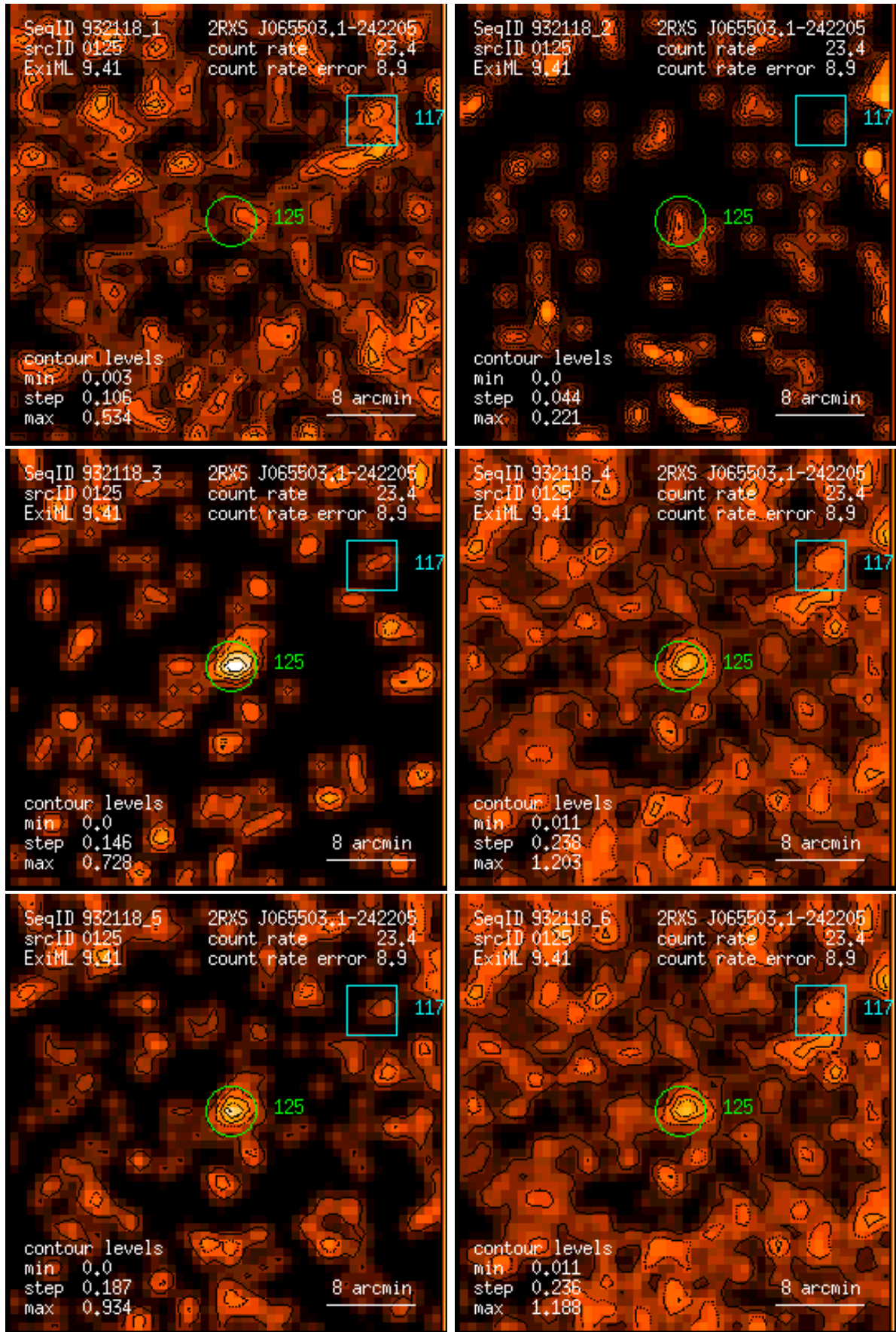
Figure 125: RASS 932118: detection 0125: band rate images, Gaussian filter: (1) PSPC channels 11 – 41, (2) 52 – 90, (3) 91 – 201, (4) 11 – 235, (5) 52 – 201, (6) 11 – 201. Broad band rates in counts/ks. Band rate contour levels in counts/ks/arcmin 2 .
