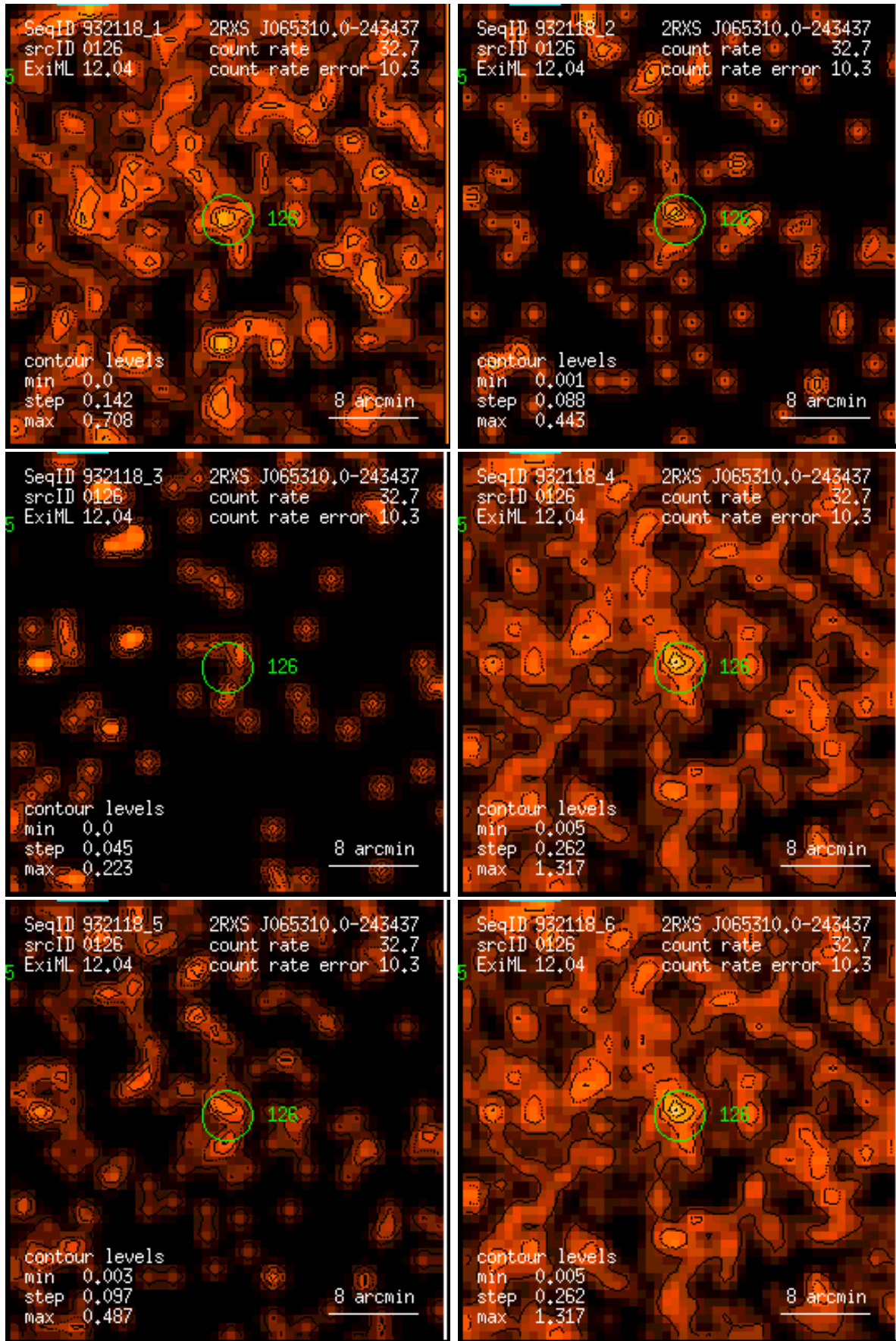
Figure 126: RASS 932118: detection 0126: band rate images, Gaussian filter: (1) PSPC channels 11 – 41, (2) 52 – 90, (3) 91 – 201, (4) 11 – 235, (5) 52 – 201, (6) 11 – 201. Broad band rates in counts/ks. Band rate contour levels in counts/ks/arcmin 2 .
