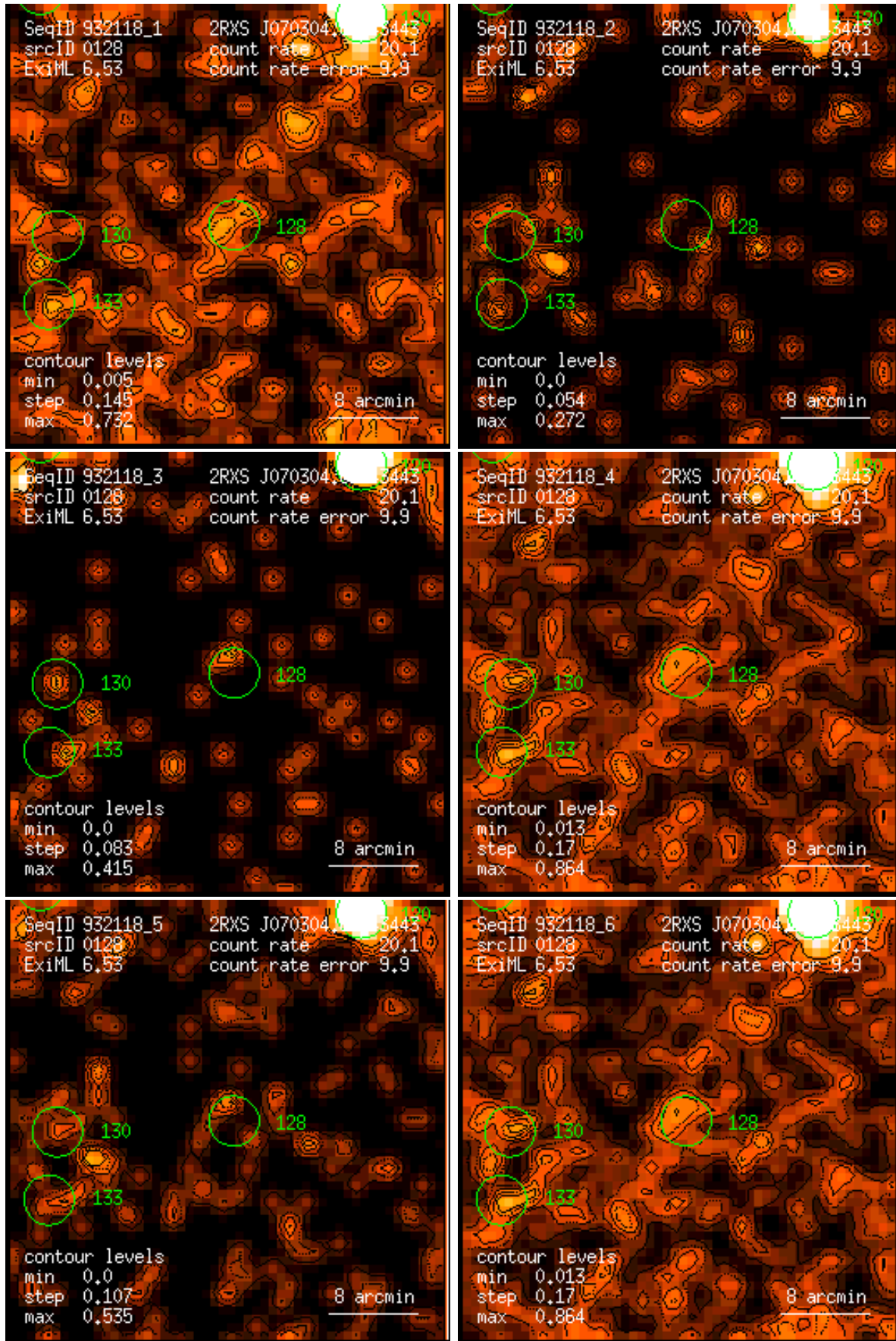
Figure 128: RASS 932118: detection 0128: band rate images, Gaussian filter: (1) PSPC channels 11 – 41, (2) 52 – 90, (3) 91 – 201, (4) 11 – 235, (5) 52 – 201, (6) 11 – 201. Broad band rates in counts/ks. Band rate contour levels in counts/ks/arcmin 2 .
