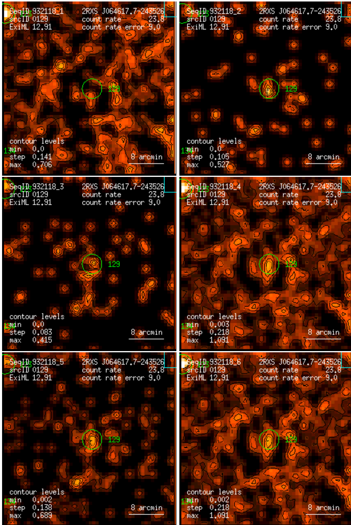
Figure 129: RASS 932118: detection 0129: band rate images, Gaussian filter: (1) PSPC channels 11 – 41, (2) 52 – 90, (3) 91 – 201, (4) 11 – 235, (5) 52 – 201, (6) 11 – 201. Broad band rates in counts/ks. Band rate contour levels in counts/ks/arcmin 2 .
