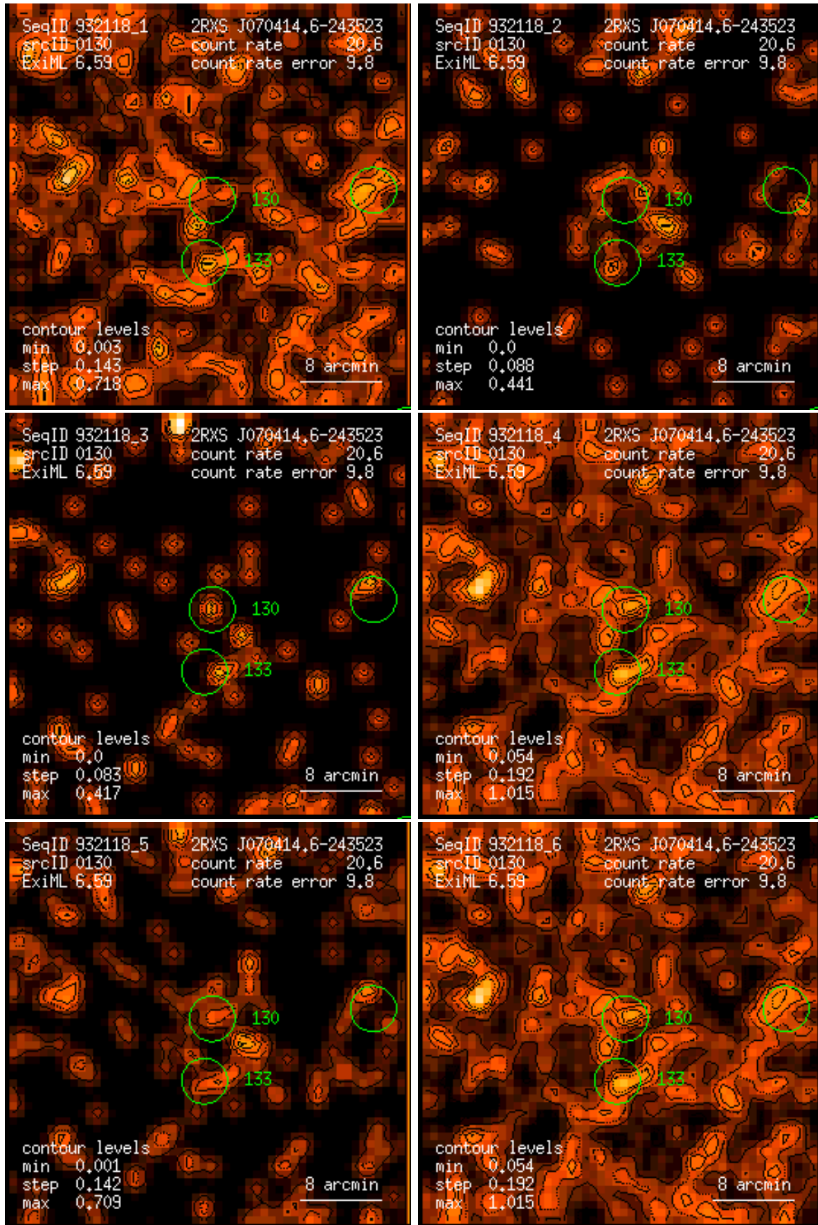
Figure 130: RASS 932118: detection 0130: band rate images, Gaussian filter: (1) PSPC channels 11 – 41, (2) 52 – 90, (3) 91 – 201, (4) 11 – 235, (5) 52 – 201, (6) 11 – 201. Broad band rates in counts/ks. Band rate contour levels in counts/ks/arcmin 2 .
