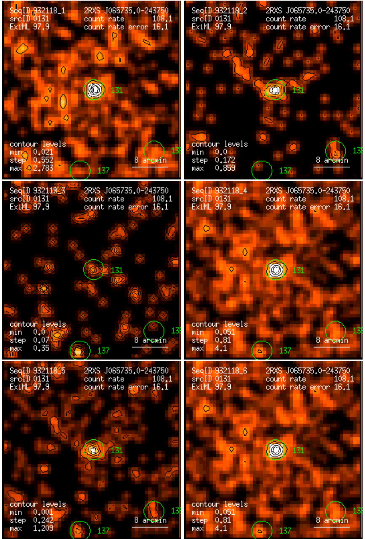
Figure 131: RASS 932118: detection 0131: band rate images, Gaussian filter: (1) PSPC channels 11 – 41, (2) 52 – 90, (3) 91 – 201, (4) 11 – 235, (5) 52 – 201, (6) 11 – 201. Broad band rates in counts/ks. Band rate contour levels in counts/ks/arcmin 2 .
