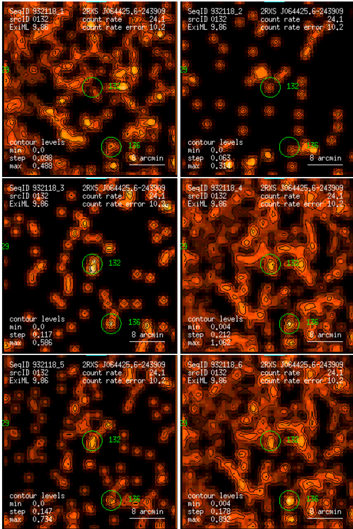
Figure 132: RASS 932118: detection 0132: band rate images, Gaussian filter: (1) PSPC channels 11 – 41, (2) 52 – 90, (3) 91 – 201, (4) 11 – 235, (5) 52 – 201, (6) 11 – 201. Broad band rates in counts/ks. Band rate contour levels in counts/ks/arcmin 2 .
