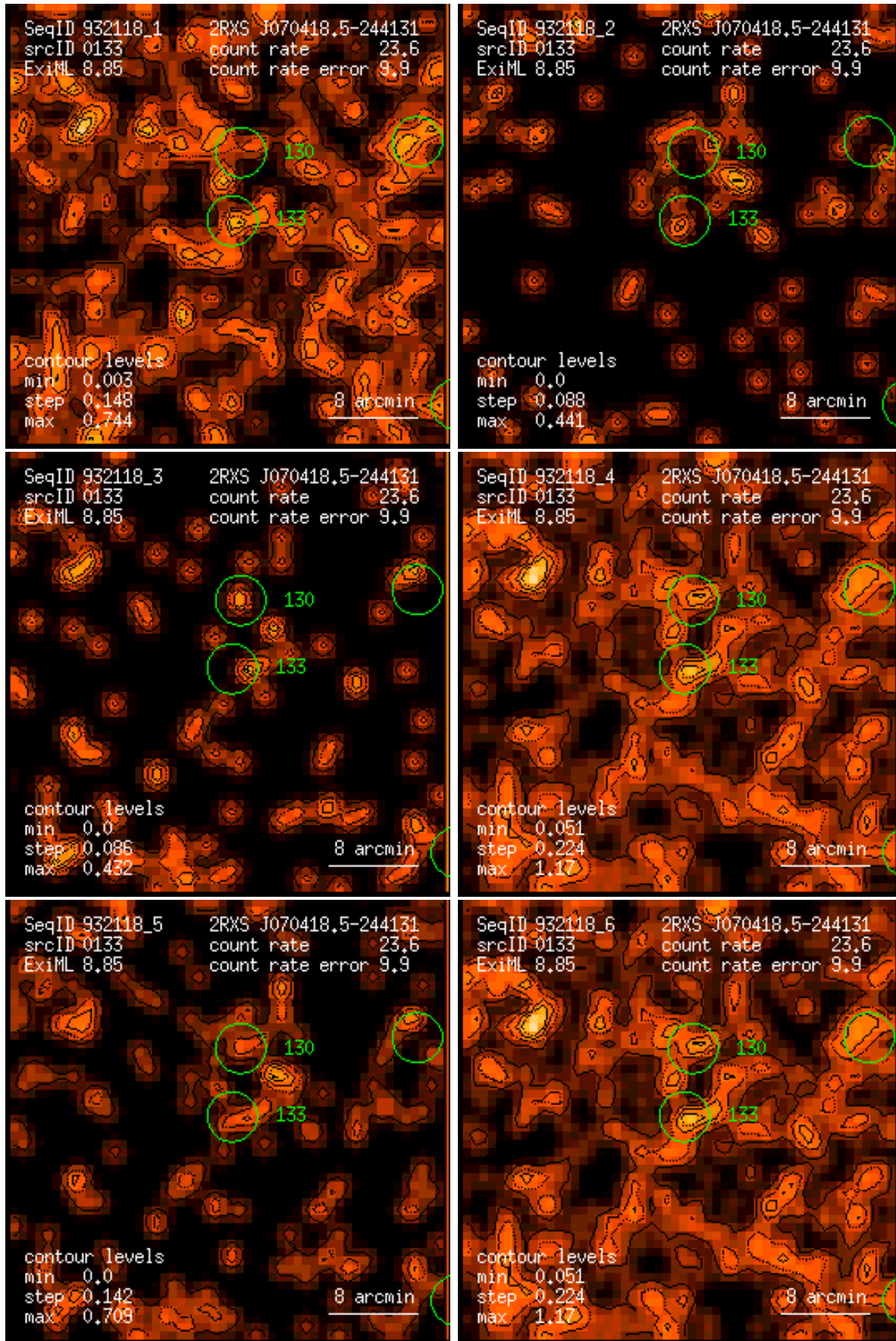
Figure 133: RASS 932118: detection 0133: band rate images, Gaussian filter: (1) PSPC channels 11 – 41, (2) 52 – 90, (3) 91 – 201, (4) 11 – 235, (5) 52 – 201, (6) 11 – 201. Broad band rates in counts/ks. Band rate contour levels in counts/ks/arcmin 2 .
