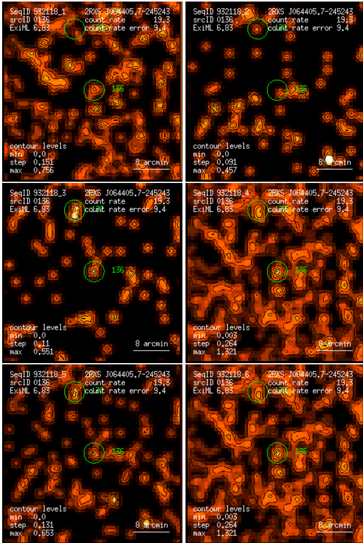
Figure 136: RASS 932118: detection 0136: band rate images, Gaussian filter: (1) PSPC channels 11 – 41, (2) 52 – 90, (3) 91 – 201, (4) 11 – 235, (5) 52 – 201, (6) 11 – 201. Broad band rates in counts/ks. Band rate contour levels in counts/ks/arcmin 2 .
