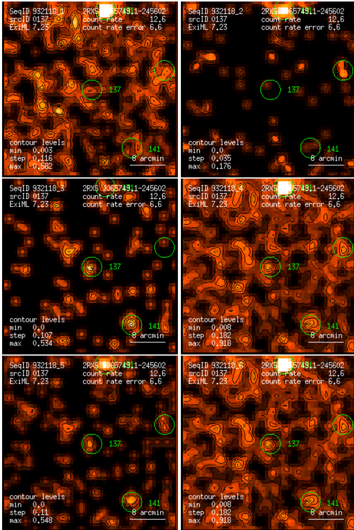
Figure 137: RASS 932118: detection 0137: band rate images, Gaussian filter: (1) PSPC channels 11 – 41, (2) 52 – 90, (3) 91 – 201, (4) 11 – 235, (5) 52 – 201, (6) 11 – 201. Broad band rates in counts/ks. Band rate contour levels in counts/ks/arcmin 2 .
