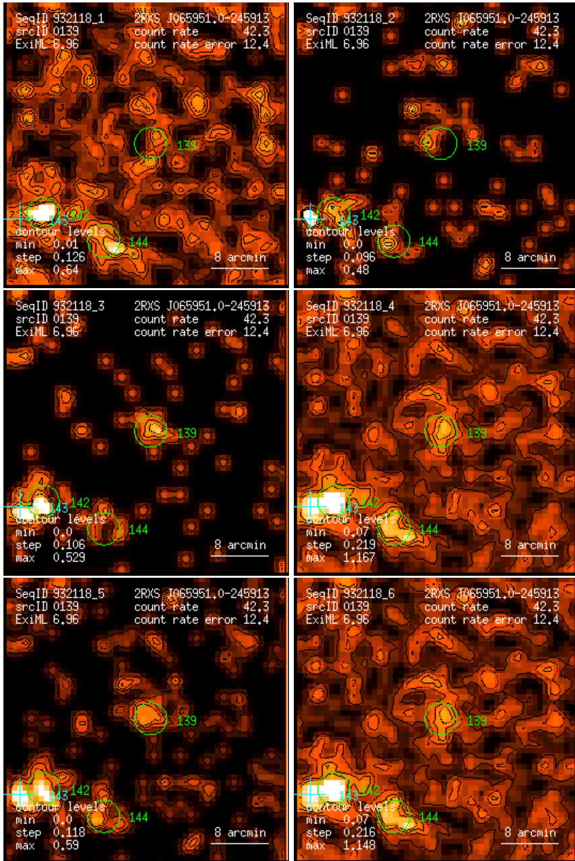
Figure 139: RASS 932118: detection 0139: band rate images, Gaussian filter: (1) PSPC channels 11 – 41, (2) 52 – 90, (3) 91 – 201, (4) 11 – 235, (5) 52 – 201, (6) 11 – 201. Broad band rates in counts/ks. Band rate contour levels in counts/ks/arcmin 2 .
