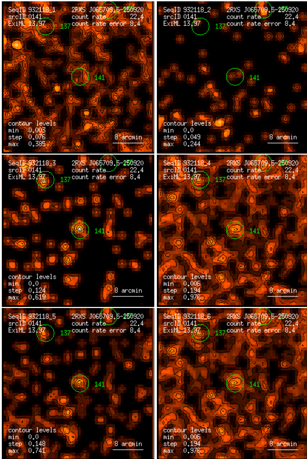
Figure 141: RASS 932118: detection 0141: band rate images, Gaussian filter: (1) PSPC channels 11 – 41, (2) 52 – 90, (3) 91 – 201, (4) 11 – 235, (5) 52 – 201, (6) 11 – 201. Broad band rates in counts/ks. Band rate contour levels in counts/ks/arcmin 2 .
