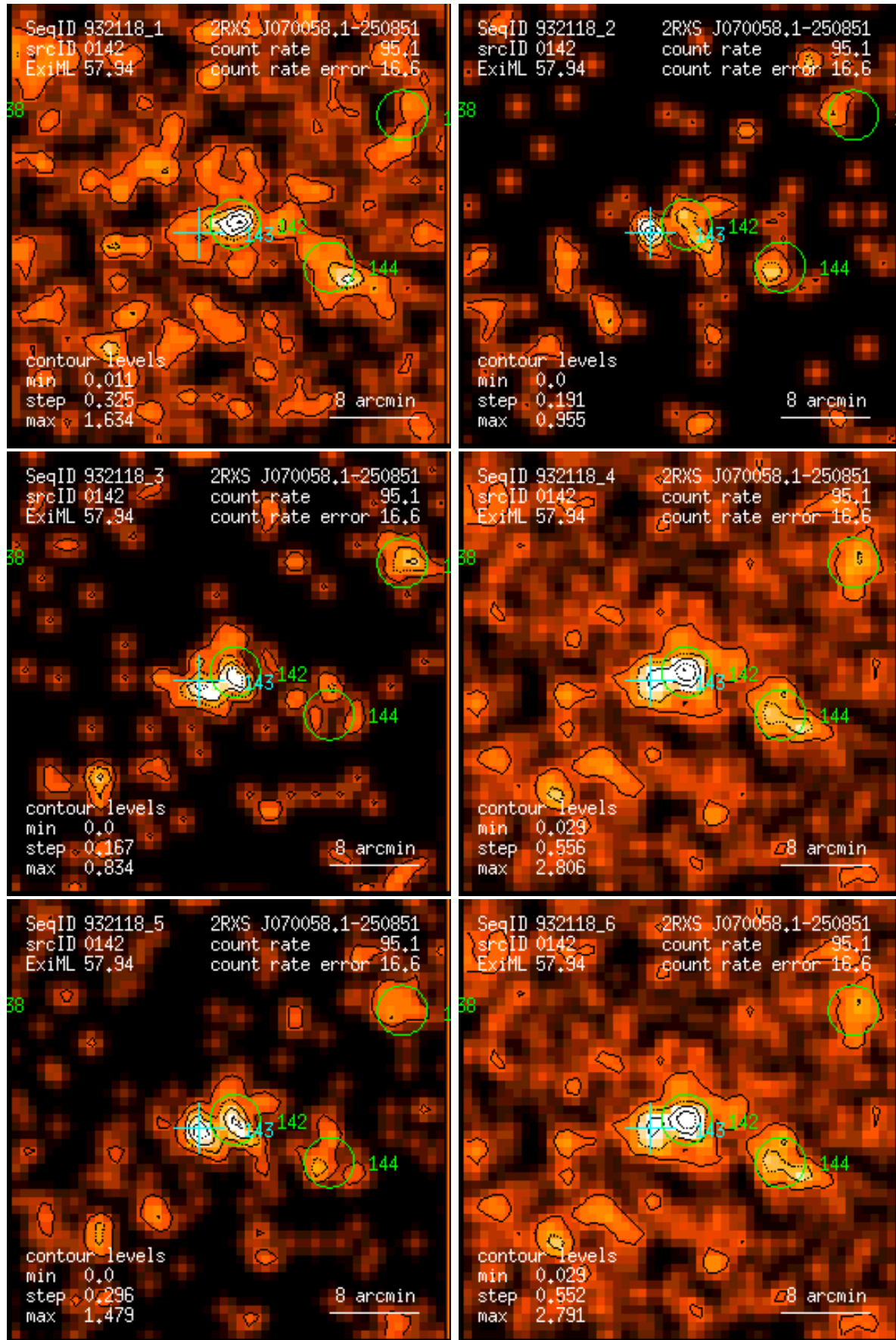
Figure 142: RASS 932118: detection 0142: band rate images, Gaussian filter: (1) PSPC channels 11 – 41, (2) 52 – 90, (3) 91 – 201, (4) 11 – 235, (5) 52 – 201, (6) 11 – 201. Broad band rates in counts/ks. Band rate contour levels in counts/ks/arcmin 2 .
