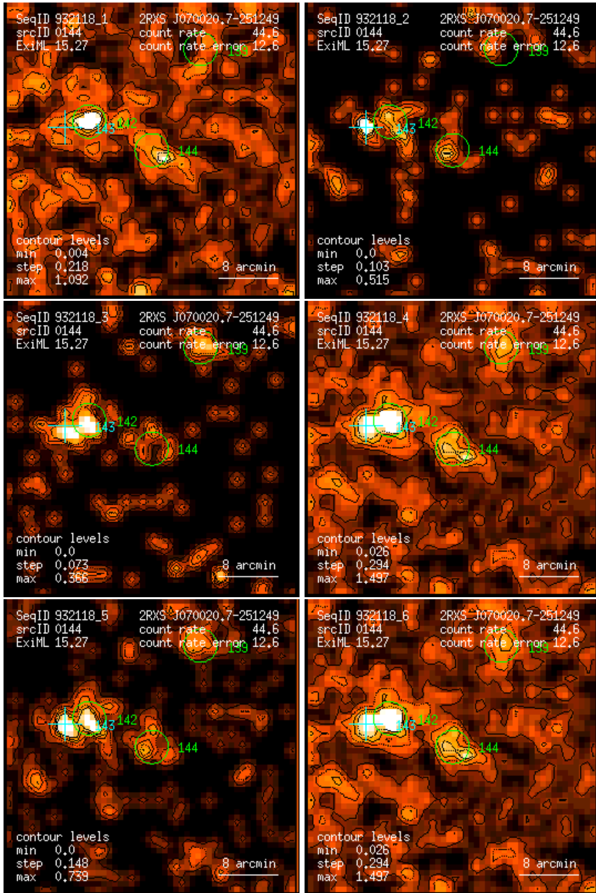
Figure 144: RASS 932118: detection 0144: band rate images, Gaussian filter: (1) PSPC channels 11 – 41, (2) 52 – 90, (3) 91 – 201, (4) 11 – 235, (5) 52 – 201, (6) 11 – 201. Broad band rates in counts/ks. Band rate contour levels in counts/ks/arcmin 2 .
