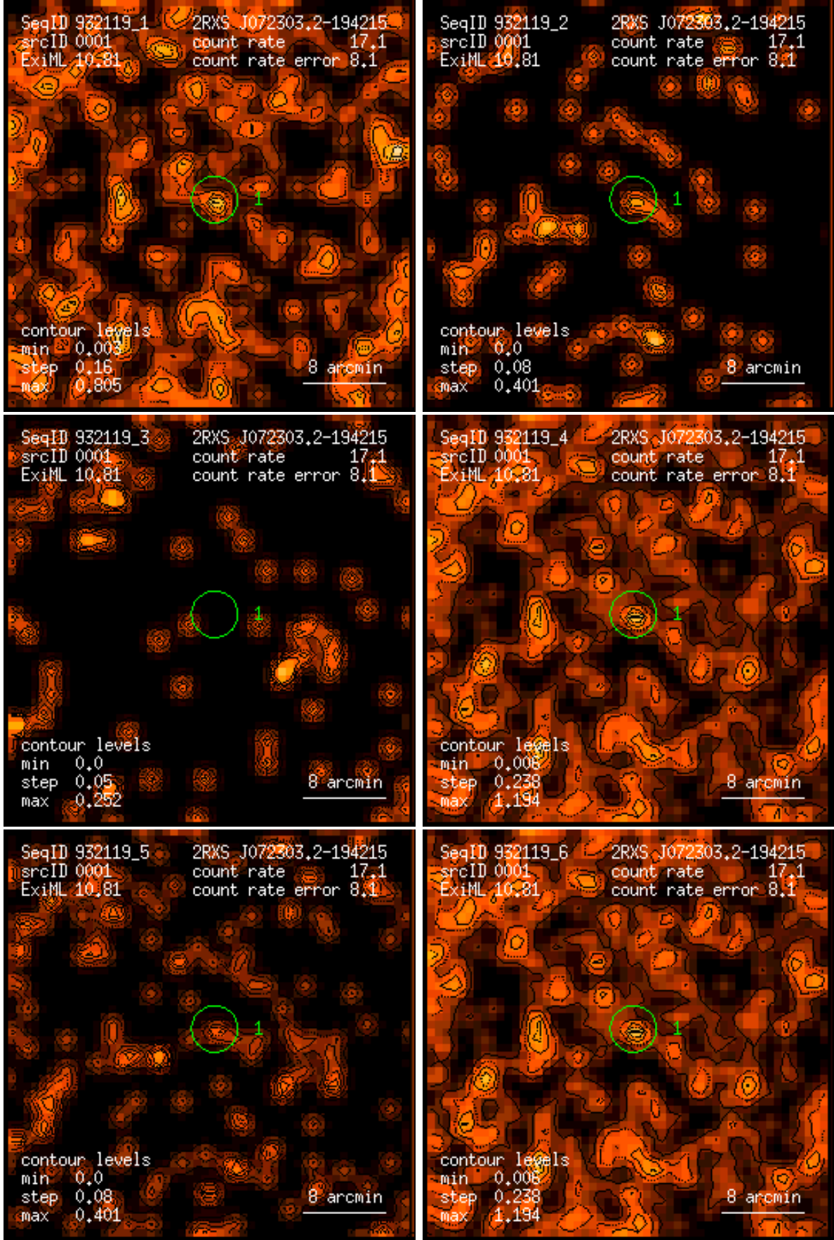
Figure 1: RASS 932119: detection 0001: band rate images, Gaussian filter: (1) PSPC channels 11 – 41, (2) 52 – 90, (3) 91 – 201, (4) 11 – 235, (5) 52 – 201, (6) 11 – 201. Broad band rates in counts/ks. Band rate contour levels in counts/ks/arcmin 2 .
