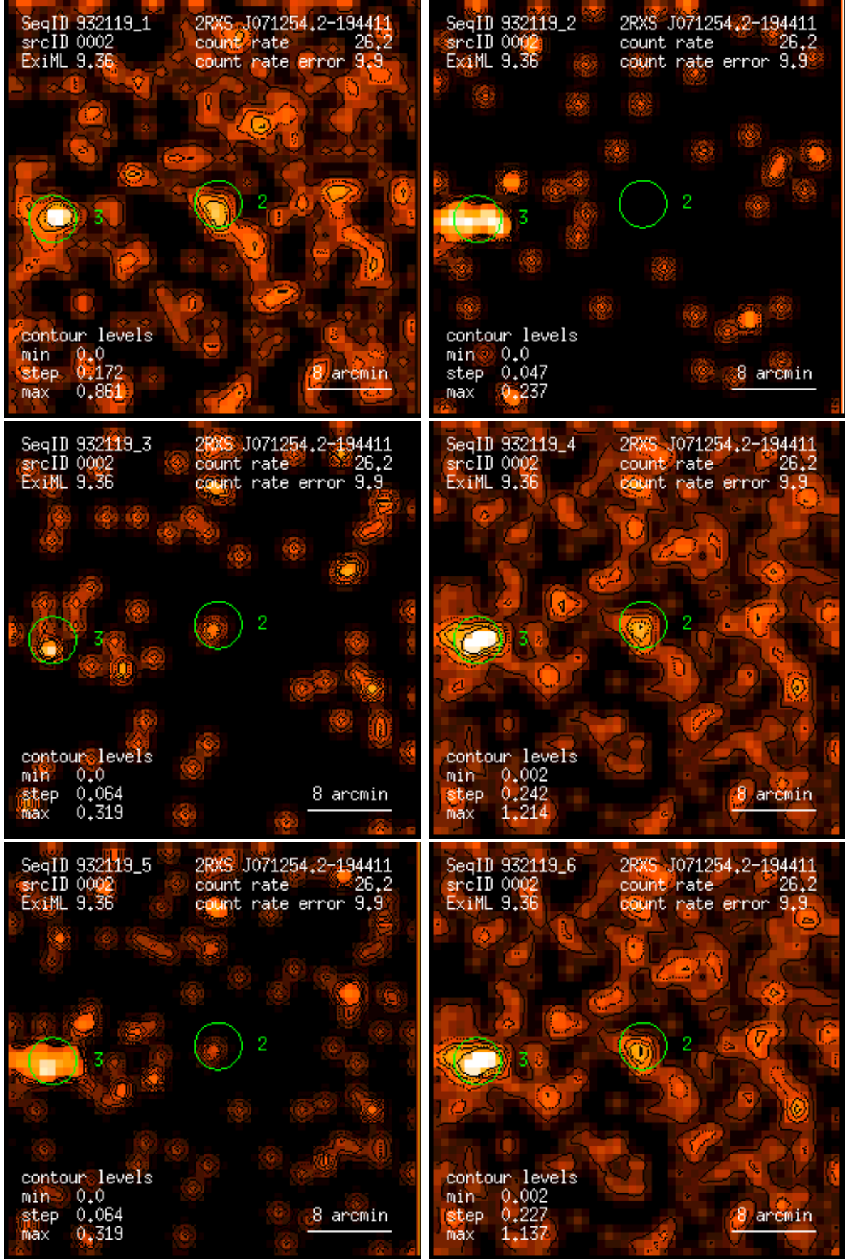
Figure 2: RASS 932119: detection 0002: band rate images, Gaussian filter: (1) PSPC channels 11 – 41, (2) 52 – 90, (3) 91 – 201, (4) 11 – 235, (5) 52 – 201, (6) 11 – 201. Broad band rates in counts/ks. Band rate contour levels in counts/ks/arcmin 2 .
