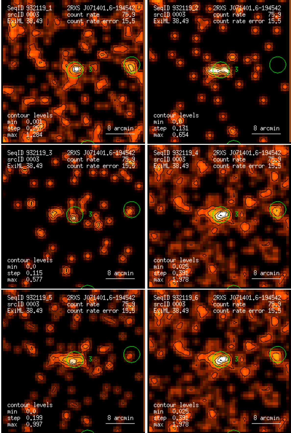
Figure 3: RASS 932119: detection 0003: band rate images, Gaussian filter: (1) PSPC channels 11 – 41, (2) 52 – 90, (3) 91 – 201, (4) 11 – 235, (5) 52 – 201, (6) 11 – 201. Broad band rates in counts/ks. Band rate contour levels in counts/ks/arcmin 2 .
