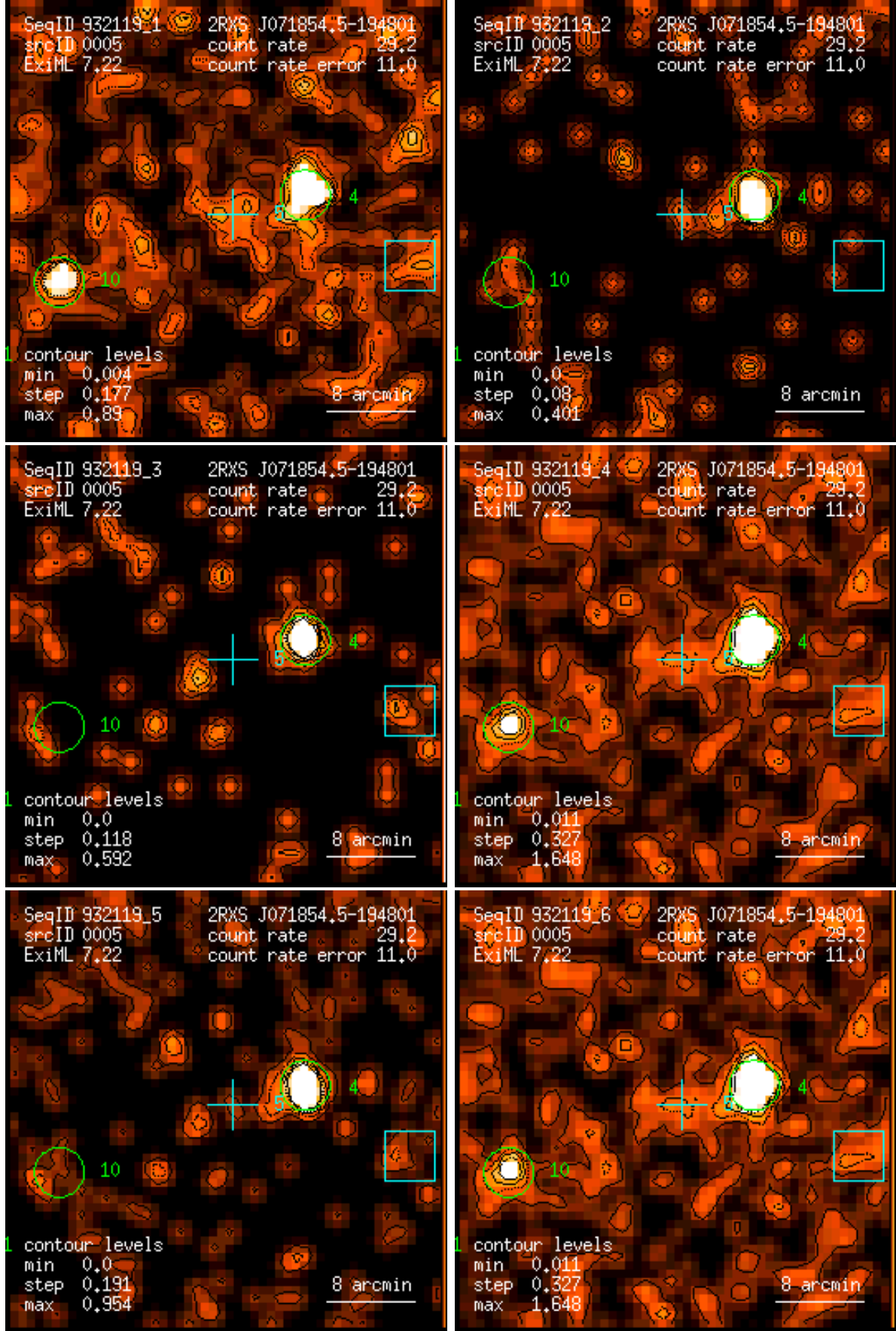
Figure 5: RASS 932119: detection 0005: band rate images, Gaussian filter: (1) PSPC channels 11 – 41, (2) 52 – 90, (3) 91 – 201, (4) 11 – 235, (5) 52 – 201, (6) 11 – 201. Broad band rates in counts/ks. Band rate contour levels in counts/ks/arcmin 2 .
